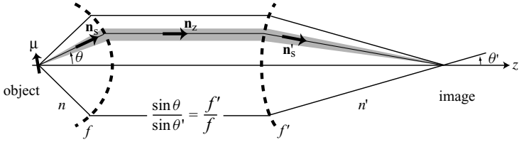
Figure 4.1 Configuration used for the calculation of the point-spread function. The source is an arbitrarily oriented electric dipole with moment \mu . The dipole radiation is collected with a high NA aplanatic objective lens and focused by a second lens on the image plane at z = 0 .
