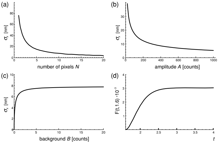
Figure 4.14 Dependence of \sigma_x on several relevant parameters for \gamma = 125 nm and dependence of F(t, \kappa) on t . (a) Plot of \sigma_x vs. number of pixels N . Other parameters: A = 500 , B = 10 , t = 5 , \Delta_a = 5.9 , \kappa = 1.6 . (b) Plot of \sigma_x vs. the amplitude of the signal A . Other parameters: B = 10 , t = 5 , \Delta_a = 5.9 , N = 10 , \kappa = 1.6 . (c) Plot of \sigma_x vs. the background level B . Other parameters: A = 500 , t = 5 , \Delta_a = 5.9 , N = 10 , \kappa = 1.6 . (d) Plot of F(t, \kappa) vs. t for \kappa = 1.6 .
