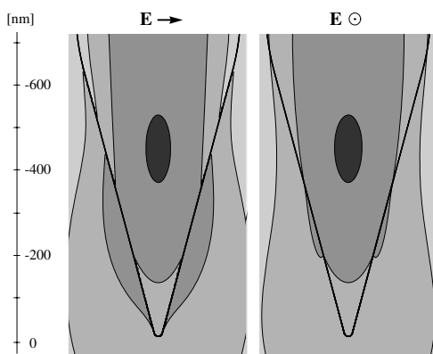
Figure 6.8 Contours of constant power density on two perpendicular planes through the center of a dielectric probe (factor of 3 between adjacent lines). The fields are excited by the HE_{11} mode (polarization indicated by symbols) incident from the upper cylindrical part. \lambda = 488 \text{ nm} , \varepsilon = 2.16 .
