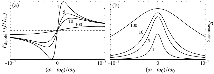
Figure 13.4 Dipole force and scattering force for sodium atoms ( 1/\gamma = 16.1 ns, \lambda_0 = 590 nm) as a function of excitation frequency \omega . The numbers in the figures indicate the value of the ratio I/I_{\text{sat}} .
