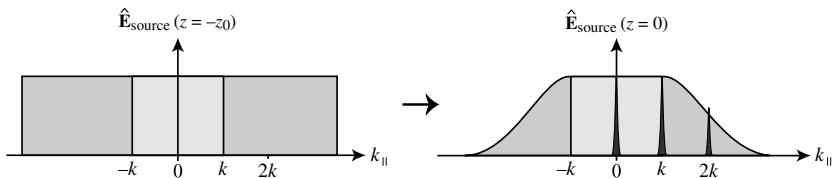
Figure 4.21 Attenuation of bandwidth of spatial frequencies upon propagation from source ( z = -z_0 ) to sample ( z = 0 ). Evanescent components ( k_{\parallel} > k ) are exponentially attenuated. The attenuation is stronger the larger k_{\parallel} is. The spatial spectrum arriving at the sample can be written as a sum over discrete spatial frequencies represented by delta functions. Only three representative spatial frequencies are depicted for illustration: \delta(k_{\parallel}) , \delta(k_{\parallel} - k) , and \delta(k_{\parallel} - 2k) .
