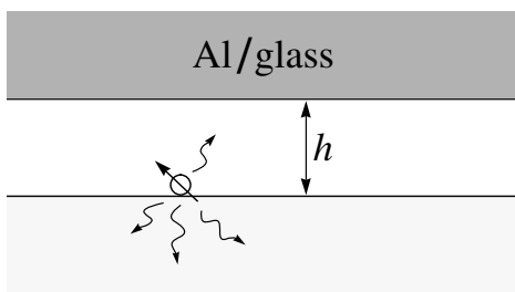
Figure 10.4 Single molecule fluorescence near planar interfaces. The molecule is located on the surface of a dielectric substrate and a metal ( \epsilon = -34.5 + i8.5 ) or a glass ( \epsilon = 2.25 ) interface is advanced from above. The applied wavelength is \lambda = 488 nm.
