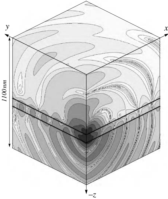
Figure 10.3 Power density of a dipole above a slab waveguide depicted at a certain time. The dipole is located at h = 20 nm and its axis is in the (x, z) -plane. \theta = 60^\circ , \lambda = 488 nm, d = 80 nm, \varepsilon_1 = 1 , \varepsilon_2 = 5 , \varepsilon_3 = 2.25 . Factor of 2 between successive contour lines.
