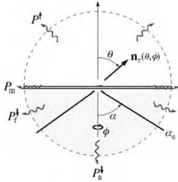
Figure 10.6 Definition of angles used for the asymptotic far-fields. The radiated power is split into the contributions P^\uparrow (radiation into upper half-space), P_a^\downarrow (radiation into allowed zone), P_f^\downarrow (radiation into forbidden zone), and P_m (radiation dissipated in the layered medium). The total rate of energy dissipation is P = P^\uparrow + P_a^\downarrow + P_f^\downarrow + P_m + P_i , with P_i being the intrinsically dissipated power.
