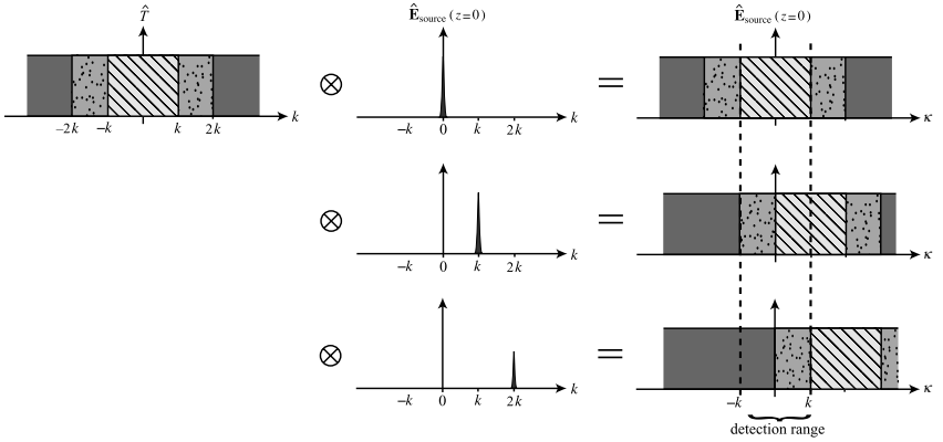
Figure 4.22 Convolution of the spatial spectra of sample transmission ( \hat{T} ) and source field ( \hat{\mathbf{E}}_{\text{source}} ). Three discrete spatial frequencies of \hat{\mathbf{E}}_{\text{source}} are shown. Convolution with \delta(k_{\parallel} - mk) shifts the spatial spectrum of \hat{T} by mk . m = 0 corresponds to a plane wave at normal incidence, m = 1 to a plane wave at parallel incidence, and m = 2 is an evanescent wave. In the far-field, the resulting spectrum of \hat{\mathbf{E}}_{\text{sample}} can only be detected in the range k_{\parallel} = [-k \dots k] . The figure illustrates that evanescent components in the source field shift the high spatial frequencies of the sample into the detection window.
