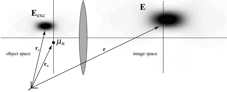
Figure 4.4 Schematic of a general set-up using a confined excitation source for sample excitation. The dipole strength \mu_n of the point source depends on the excitation field \mathbf{E}_{\text{exc}} . The point-spread function defined by the field \mathbf{E} in the image space depends on the nature of the interaction between \mu_n and \mathbf{E}_{\text{exc}} , and on the relative coordinates \mathbf{r}_n - \mathbf{r}_s .
