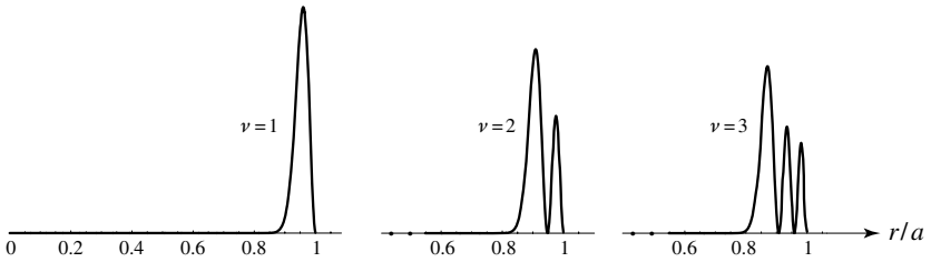
Figure 11.7 Radial energy distribution of TM modes with angular momentum mode number l = 120 . The microsphere has a dielectric constant of \varepsilon = 2.31 . The radial mode number \nu indicates the number of energy maxima in the radial direction.
