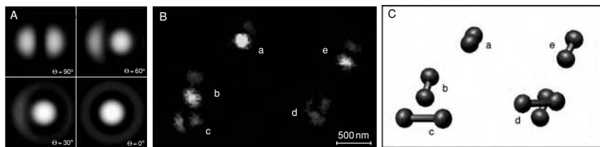
Figure 9.15 (A) Calculated fluorescence rate patterns for a focused, radially polarized excitation beam. The out-of-plane orientation of the probing molecular dipole moment is indicated by the angle \Theta ( \Theta = 0 corresponds to an in-plane molecule, i.e. oriented perpendicular to the optical axis). (B) Corresponding experimental patterns obtained with molecules that are randomly oriented in a thin polymer film. (C) Reconstructed dipole orientations. From [25].
