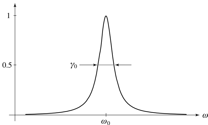
Figure 8.7 Lorentzian lineshape function as defined by the expression in brackets in Eq. (8.133).
