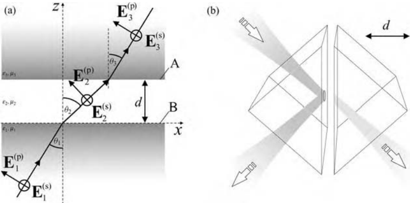
Figure 2.7 Transmission of a plane wave through a system of two parallel interfaces. In frustrated total internal reflection (FTIR), the evanescent wave created at interface B is partly converted into a propagating wave by the interface A of a second medium. (a) Configuration and definition of parameters. A, B: interfaces between media 2, 3 and 1, 2, respectively. The reflected waves are omitted for clarity. (b) Experimental set-up to observe frustrated total internal reflection.
