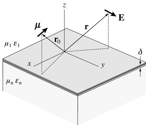
Figure 10.1 Configuration of the dipole problem. The dipole is located at \mathbf{r}_0 = (x_0, y_0, z_0) and the planar interfaces are characterized by z = \text{const} . The surface of the topmost layer coincides with the coordinate origin. The properties of the upper and lower half-spaces are designated by the index 1 and n , respectively.
