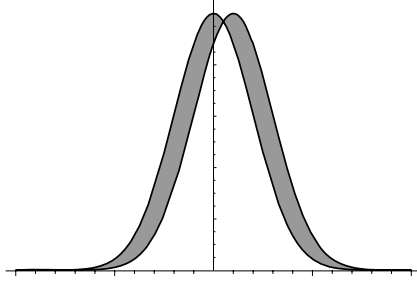
Figure 4.13 Two Gaussians displaced by a small amount. It is obvious that the main contribution to the differences between the two curves (shaded in gray) occurs where the slope is large. This is expressed in Eq. (4.58).
