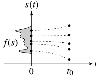
Figure 14.3 Newton's equations of motion map each phase-space point s at time t = 0 into a phase-space point at time t_0 . The dipole moment at time t_0 can be expressed as \boldsymbol{\mu}[s(t_0)] = \boldsymbol{\mu}[s(0), t_0] = \boldsymbol{\mu}[s, t_0] and its ensemble average at time t_0 is determined by the initial distribution function f(s) .
