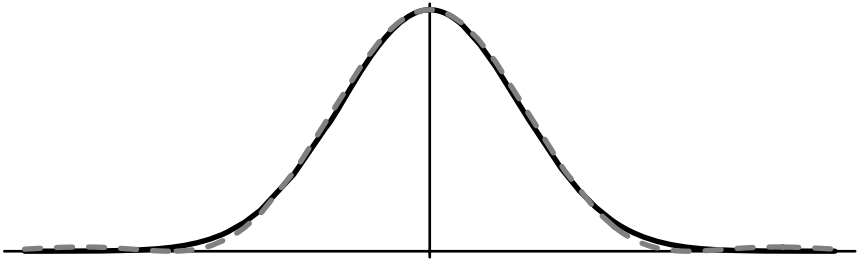
Figure 4.12 Similarity of the Airy function and a Gaussian. The deviations are negligible for noisy data.
