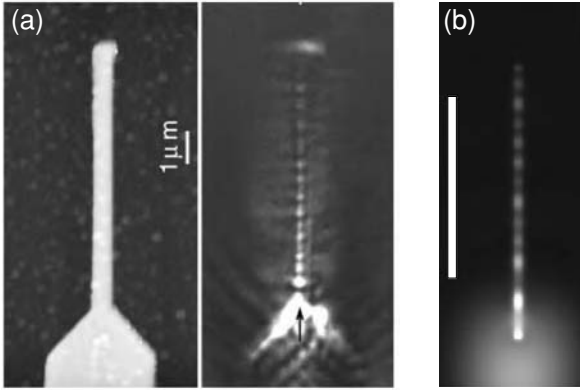
Figure 12.15 SPP waveguides. (a) Propagation, reflection and interference of surface plasmons guided by a gold nanowire with a width of \lambda/4 ( \lambda = 800 nm). Left: shear-force topography, right: optical image recorded with a photon scanning tunneling microscope (PSTM). From [25]. (b) Simulation of surface plasmon propagation on a finite length gold rod showing a similar standing wave pattern. Scale bar 1 \mu\text{m} . From [26].
