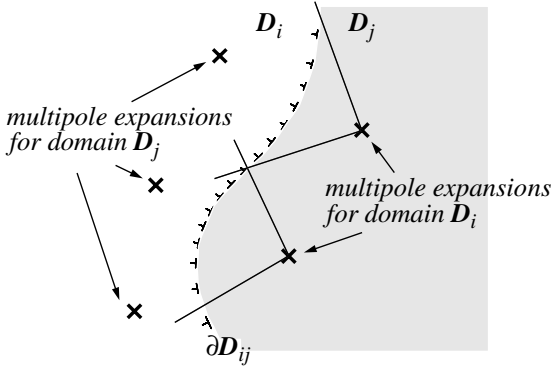
Figure 15.1 Schematic principle of the multiple multipole method. Multipole expansions located in domain D_j approximate the electromagnetic field inside domain D_i and vice versa. On each side of the boundary \partial D_{ij} the field close to a point on the interface is defined mainly by the closest multipole (indicated by the sectors for the field in domain D_i ).
