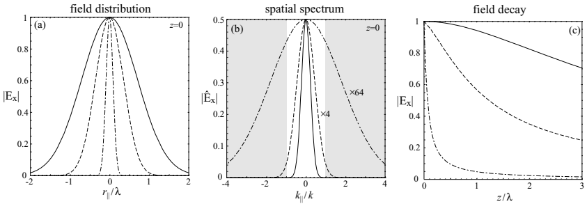
Figure 4.18 (a) Gaussian field distributions with different confinements in the source plane z=0 : w_0 = \lambda (solid curve), w_0 = \lambda/2 (dashed curve) and w_0 = \lambda/8 (dash-dotted curve). (b) Spectrum of spatial frequencies corresponding to the field distributions in (a). The shaded area denotes the range of spatial frequencies associated with evanescent fields. The better the confinement of the optical field is the broader the spectrum of spatial frequencies will be. (c) Field decay along the optical axis z corresponding to the field distributions in (a). The better the confinement in the source plane is the faster the field decay will be.
