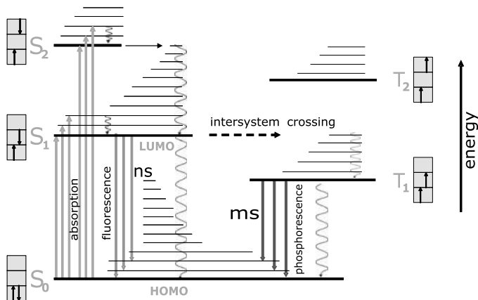
Figure 9.1 Energy level diagram of an organic molecule. The electronic singlet states S_0 , S_1 , S_2 are complemented by a manifold of vibrational states. Excitation of the molecule is followed by fast internal relaxation to the vibronic ground state of the first excited state (Kasha rule). From here the molecule can decay either radiatively (fluorescence, straight lines) or non-radiatively (dissipation to heat, wavy lines). Since the radiative decay often ends up in a vibrational state, the fluorescence is red-shifted with respect to the excitation (Stokes shift). Spin-orbit coupling leads to rare events of intersystem crossing (dashed arrow) into a triplet state with a long lifetime which relaxes through phosphorescence or non-radiatively.
