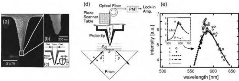
Figure 6.39 Plasmon fiber probe. (a)–(c) SEM images and sketch of the optical probe. (d) Scanning tunneling optical microscopy set-up used in the study. (e) Wavelength dependence of the light picked up by the plasmon probe. The inset shows a comparison of the metal coated to a bare fiber probe. Adapted from [75].
