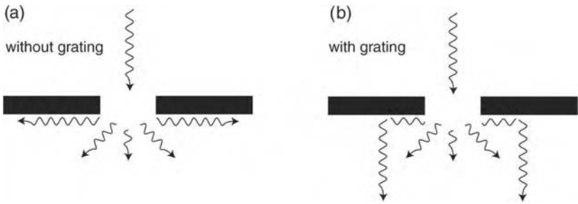
Figure 6.19 Improving the directionality of light emission by a grating fabricated on the exit side of a small aperture. (a) Without the grating radiation diffracts into all directions. (b) The grating delocalizes the near-field and converts it into directional radiation.
