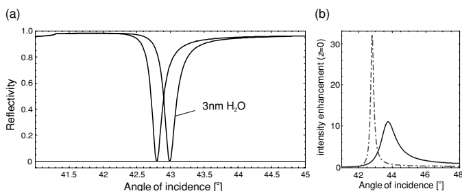
Figure 12.9 Surface plasmons used in sensor applications. (a) Calculated shift of the SPP resonance curve induced by a 3 nm layer of water ( n = 1.33 ) adsorbed on a 53 nm silver film. (b) Intensity enhancement near the metal surface as a function of the angle of incidence in the Kretschmann configuration. For silver ( \epsilon_1 = -18.2 + 0.5i , dash-dotted line) and gold ( \epsilon_1 = -11.6 + 1.2i , solid line) at a wavelength of 633 nm we observe a maximum intensity enhancement of \sim 32 and \sim 10 , respectively.
