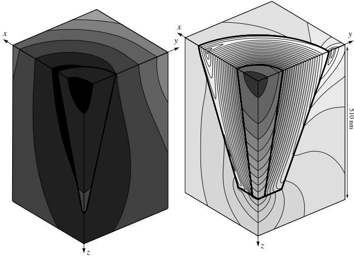
Figure 6.10 Contour lines of constant |\mathbf{E}|^2 on three perpendicular planes through a dielectric probe (left) and an aperture probe (right) (factor of 4 between successive lines). \lambda = 488 \text{ nm} , \epsilon_{\text{core}} = 2.16 , \epsilon_{\text{coat}} = -34.5 + i8.5 . The exciting \text{HE}_{11} mode is polarized along the x -direction.
