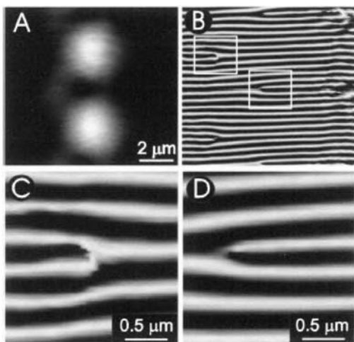
Figure 5.22 Evanescent fields above the \text{Si}_3\text{N}_4 channel waveguide shown in Fig. 5.21(A). Linearly polarized light has been coupled in the channel waveguide to excite the lowest TE and TM modes simultaneously. (A) Measured amplitude of the optical field inside the waveguide. A clear beating pattern is observed. (B) Measured phase distribution of the optical field. The cosine of the phase is shown. Several phase singularities are apparent. (C) Close-up of the square region (left) indicated in (B). The phase singularity has a topological charge +1 . (D) Close-up of the square region (right) indicated in (B). The phase singularity has a topological charge -1 . From [40].
