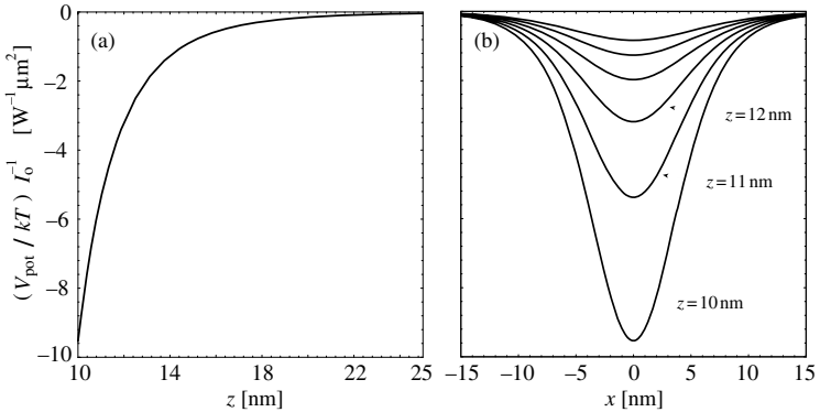
Figure 13.13 Trapping potential V_{\text{pot}} along the tip axis (a) and along a transverse direction at z = r_t + r_0 beneath the tip. An enhancement factor of f = 3000 is assumed. The radii of tip and particle are r_t = r_0 = 5 nm. The dielectric constants of particle and environment are \varepsilon = 2.5 and \varepsilon_s = 1.77 (water), respectively. The forces are normalized with k_B T and the incident intensity I_0 .
