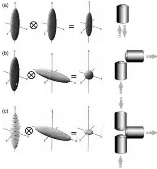
Figure 5.3 Point-spread function engineering. (a) Standard epi-illumination confocal microscopy. (b) Confocal theta configuration. (c) 4\pi confocal theta configuration. Adapted from [3].
