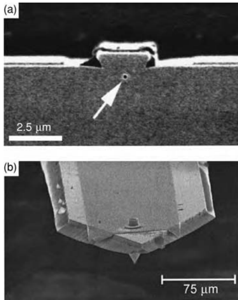
Figure 6.31 (a) Small-aperture laser diode. From [56]. (b) VCSEL integrated into a GaAs cantilever. From [57].
