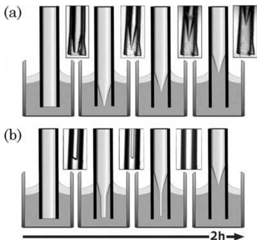
Figure 6.2 Schematic view of the time evolution of the tube-etching process. The insets show in situ video frames of the etching process. Cleaved fibers are dipped into a 40% HF solution with an organic overlayer ( p -xylene or iso-octane). The etching proceeds along different pathways whether or not the polymer fiber cladding is permeable to HF. In the case of a non-permeable cladding the tip forms at the end of the fiber and keeps its shape while shortening inside the tube (a). In the second case the tip forms at the meniscus between HF and the organic overlayer (b). From [5].
