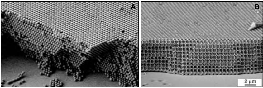
Figure 11.1 Fabrication of silicon photonic bandgap crystals. (a) Template produced by 855 nm silica spheres deposited on a Si wafer. (b) Photonic crystal obtained after filling the interstitial spaces with high-index Si and removing the template by wet etching. From [3].
