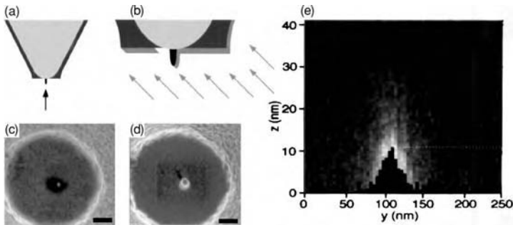
Figure 6.37 Tip-on-aperture geometry: (a), (b) Sketch of the fabrication process including mini tip formation and subsequent metal coating. (c), (d) SEM images of the resulting structure corresponding to the sketches in (a) and (b). (e) The fluorescence response of a fluorescent bead under a mini tip. The strong vertical confinement is indicative of a high lateral resolution. Adapted from [71].
