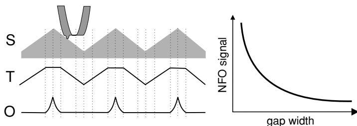
Figure 7.12 Near-field optical imaging on a sample with large topographic variations. Left panel: S, sample profile; T, apparent topography measured by the probe; O, detected optical signal resulting from the particular probe-sample distance dependence (right panel).
