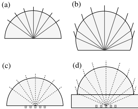
Figure 5.7 Solid immersion lens (SIL) configurations. In (a), a hemispherical lens increases resolution by \sim n . (b) A Weierstrass optic, or super-SIL, has a resolution increase of \sim n^2 . Two types of imaging modes, surface SIL microscopy (c) and subsurface SIL microscopy (d).
