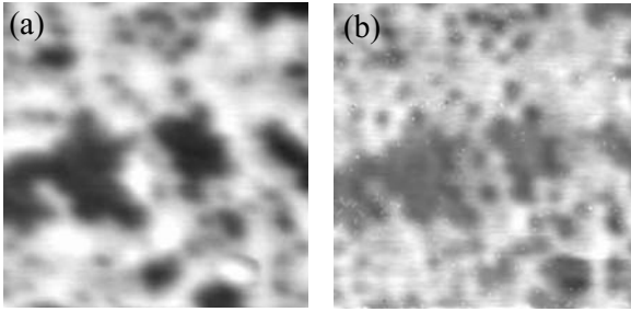
Figure 4.23 Images of a latex sphere projection pattern recorded by scanning near-field optical microscopy. In (a) detection is restricted to low spatial frequencies, whereas in (b) only the high spatial frequencies are sampled.
