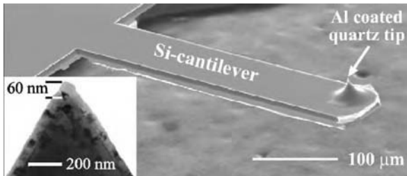
Figure 6.29 SEM image of a silicon cantilever with integrated aluminum-coated quartz tip. The inset shows a TEM image of the tip. The tip is completely covered with 60 nm of aluminum, yet is still transmissive for light. From [52].
