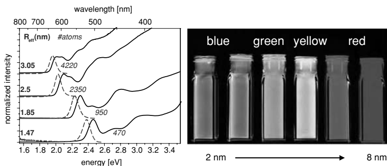
Figure 9.5 Spectral response of semiconductor nanocrystals with different sizes. Left panel: Emission spectra (dashed) and excitation spectra. Right panel: Emission from a series of nanocrystal solutions with increasing particle size excited simultaneously by a UV lamp. Courtesy of Hans Eisler.
