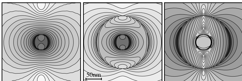
Figure 6.18 Contours of constant |\mathbf{E}|^2 (factor of 3^{1/2} between successive lines) in the aperture planes of three aperture probes with different coating thicknesses. Left: Infinite coating. Middle: Finite coating, the field is dominated by the flux emitted by the aperture. Right: Finite coating, the field is dominated by the flux from the outside coating surface.
