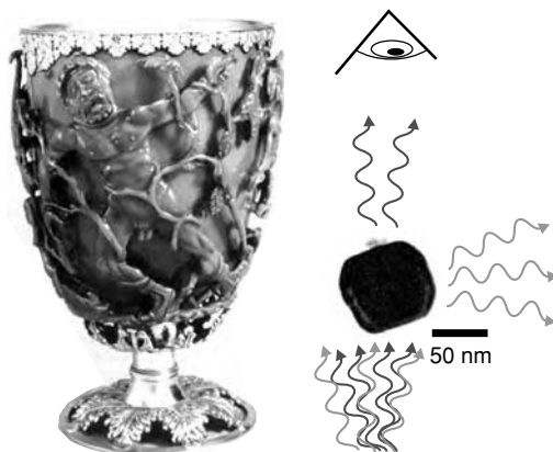
Figure 12.20 Ancient Roman Lycurgus cup illuminated by a light source from behind. Light absorption by the embedded gold/silver alloy particles (right) leads to a red color of the transmitted light whereas scattering at the particles yields a greenish color as indicated to the right. From D. J. Borber and I. C. Freestone, Archeometry 32 , 1 (1990), with permission.
