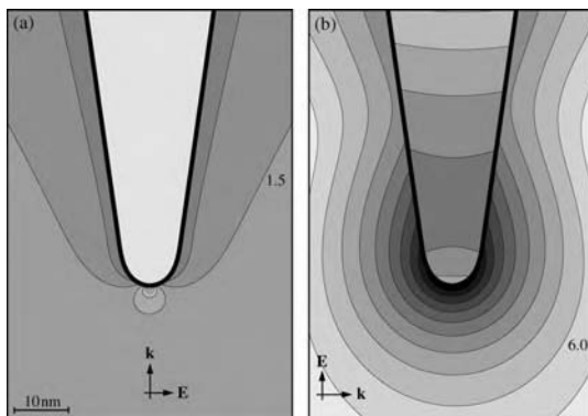
Figure 6.32 Near-field of a gold tip (5 nm tip radius) in water illuminated by two different monochromatic waves at \lambda = 810 nm. Direction and polarization of the incident wave are indicated by the \mathbf{k} and \mathbf{E} vectors. The figures show contours of E^2 (factor of 2 between successive lines). The field in (b) is almost axially symmetric in the vicinity of the tip.
