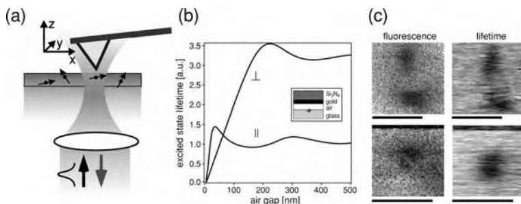
Figure 5.27 (a) Sketch of an energy transfer microscope with single-molecule sensitivity and excitation with picosecond laser pulses. (b) Excited state lifetime as a function of the gapwidth in a system of stratified layers that mimics the local geometry under the AFM tip. The dipolar emitter is located inside a 20 nm thick PMMA layer. For both the perpendicular and the in plane orientation of the dipole moment a sharp decrease of the lifetime towards a zero air gap is observed. (c) Fluorescence rate and excited state lifetime of individual molecules as a gold-coated \text{Si}_3\text{N}_4 tip (upper row) or a bare tip (lower row) is scanned over it. Adapted from [50, 51].
