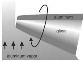
Figure 6.21 Self-aligned formation of an aperture by thermal evaporation. The evaporation takes place at an angle slightly from behind while the tip is being rotated. Adapted from [17].
