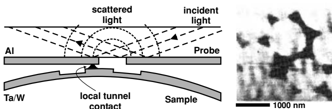
Figure 5.25 Reflection-mode SNOM. A subwavelength aperture (left) is illuminated by a waveguide mode in a glass slab. The scattering from the aperture is recorded as a function of the local environment of the aperture. Right: scan image of a latex sphere projection pattern showing subwavelength features. From [49].
