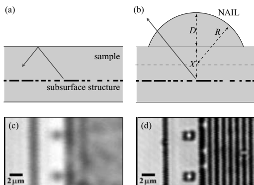
Figure 5.8 Subsurface imaging using a numerical aperture increasing lens (NAIL). (a) In a high-index material, light rays emanating from subsurface structures can undergo total internal reflection thereby reducing the NA of an imaging system. (b) Addition of a SIL enlarges the NA up to NA = n . (c, d) Comparison of images of an electronic circuit in silicon taken with and without NAIL. From [18] with permission (© 2002 IEEE).
