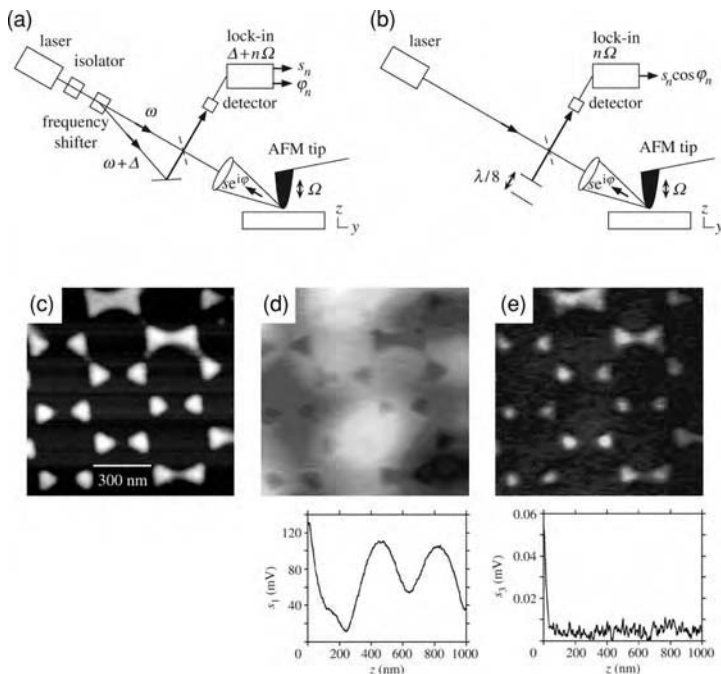
Figure 5.15 Set-ups for scattering-type scanning near-field optical microscopy using heterodyne (a) and homodyne (b) detection. Imaging example of scattering-type scanning near-field optical microscopy with demodulation. (c) Topography of a latex sphere projection pattern. (d) Upper panel: scattered light image at the fundamental oscillation frequency of the cantilever. Lower panel: approach curve showing strong interference fringes due to remaining far-field contributions. (e) Upper panel: scattered light image at the third harmonic of the cantilever. Lower panel: approach curve recorded on the third harmonic of the cantilever oscillation frequency showing a clean near-field signal. From [32].
