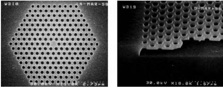
Figure 11.5 Top view and cross-section of a 2D photonic crystal with a single central defect. The crystal consists of a microfabricated hexagonal array of air holes in InGaAsP and the defect is introduced by a filled central hole. From [7].
