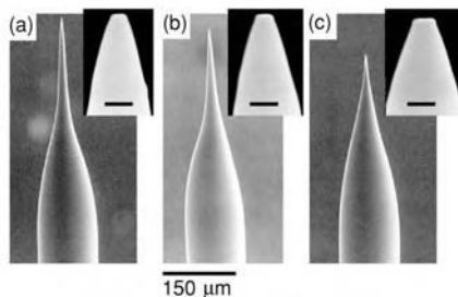
Figure 6.6 Scanning electron microscopy images of pulled glass fibers sputtered with 20 nm of gold. The insets show magnifications of the respective tip apex. There is a trend that the shorter the tip and therefore the larger the opening angle is, the more pronounced is the plateau that occurs at the apex. This plateau defines the smallest possible aperture that can be achieved after metal coating.
