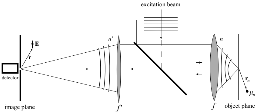
Figure 4.8 Schematic of an inverted confocal microscope. In this set-up, the light path is held fixed whereas the sample is scanned in three dimensions. A beam-splitter divides the excitation path and detection path into two separate arms. A laser beam is focused into the sample by a high NA objective lens to provide a spatially confined excitation source. The response of the sample is collected by the same objective lens and focused onto a pinhole in front of a detector.
