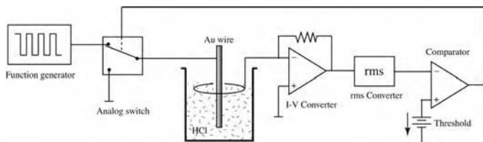
Figure 6.35 Schematic of an AC etching circuit for gold tips. The etching voltage is automatically switched off after drop-off. The circuit also works for other tip materials if HCl is replaced with a suitable etching solution. See text for details.
