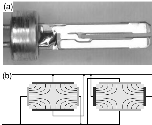
Figure 7.5 Quartz tuning fork: (a) Enlarged photograph. Dimensions of the quartz element shown are 5870 \times 1380 \times 220 \mu\text{m} . (b) Connection scheme of a quartz tuning fork for a cut perpendicular to the prongs. Adapted from [17].
