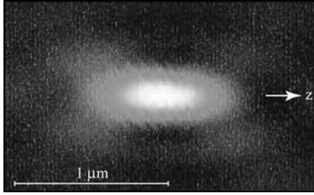
Figure 4.9 Total point-spread function (PSF) measured by scanning a gold particle through the laser focus and detecting the scattered intensity at each position. From Ref. [9].
