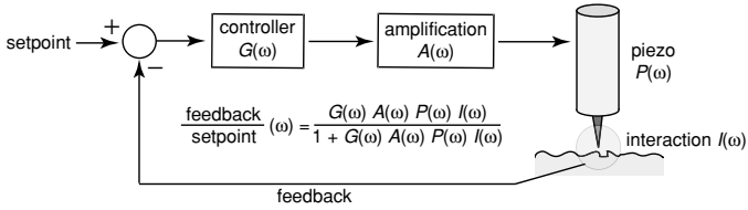
Figure 7.1 Characteristic diagram of a feedback loop employed in scanning probe microscopy. Ideally, the measured interaction signal corresponds to the externally defined setpoint. The speed and stability of the feedback loop depend on the parameters of the controller G(\omega) .
