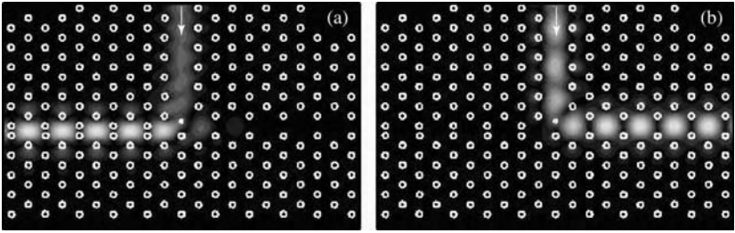
Figure 11.4 2D photonic crystal diplexer. A waveguide T-junction is formed by dislocations and removal of elements. High frequencies are deflected to the left and low frequencies are deflected to the right. The figure shows the computed optical intensity for (a) \omega = 0.956\pi c/d and (b) \omega = 0.874\pi c/d , with d being the lattice constant. From [6].
