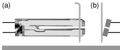
Figure 7.10 Tuning fork operated in the normal force mode. The tuning fork is aligned parallel to the sample while the probe is oscillating perpendicularly. (a) Side view, (b) front view. The fork is slightly tilted in order not to affect the second arm.
