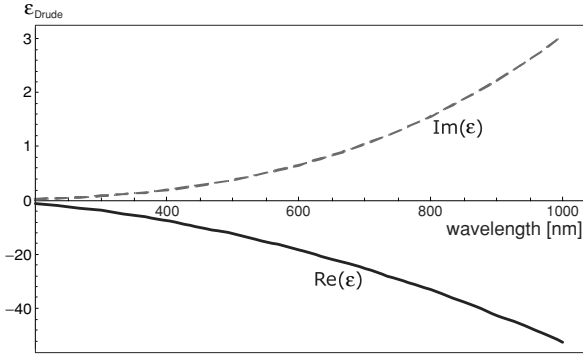
Figure 12.1 Real and imaginary part of the dielectric constant for gold according to the Drude–Sommerfeld free-electron model ( \omega_p = 13.8 \times 10^{15} \text{ s}^{-1} , \Gamma = 1.075 \times 10^{14} \text{ s}^{-1} ). The solid line is the real part, the dashed line is the imaginary part. Note the different scales for real and imaginary parts.
