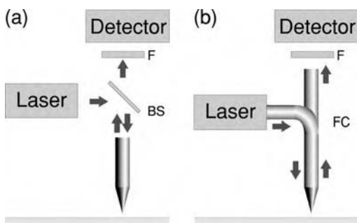
Figure 5.24 Concept of near-field microscopy in the “double-pass” mode. The probe is used both for excitation and for collection. Implementation with (a) an external beamsplitter and (b) a y-shaped fiber coupler.
