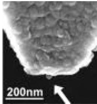
Figure 6.25 Aperture formation by laser-thermal oxidation. SEM image of an aluminum coated AFM cantilever whose tip apex was exposed for 10 s to a 488 nm laser beam at 2.5 \text{ mW}/\mu\text{m}^2 . The silicon nitride tip can be seen protruding from the otherwise flat end-face of the tip. Adapted from [44].
