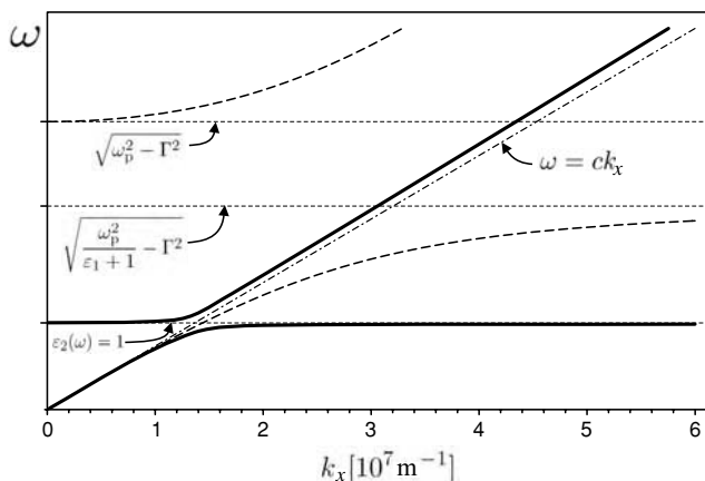
Figure 12.5 Dispersion relation of surface plasmon polaritons at a gold/air interface. The solid line is the dispersion relation that results from a dielectric function accounting for a single interband transition. The dashed line results from using a Drude type dielectric function. The dash-dotted straight line is the light line \omega = c \cdot k_x in air.
