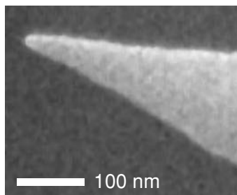
Figure 6.36 Gold tip etched from a gold wire according to the method described in the text. Radius of curvature at the tip is about 10 nm.
