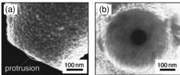
Figure 6.26 Scanning electron micrographs of (a) a side view and (b) an overhead view of an aperture with a diameter of 100 nm produced by aperture punching. Adapted from [46].
