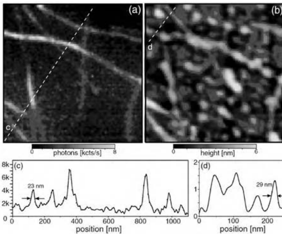
Figure 5.13 Field-enhanced near-field Raman scattering. (a) Raman scattering image acquired at \nu = 2615 \text{ cm}^{-1} and (b) shear-force topography of a sample of single-walled carbon nanotubes on a glass substrate. The topography shows that the nanotubes are covered with condensed water droplets. The line cuts (c) and (d) are taken along the respective dashed white lines in (a) and (b). From [31].
