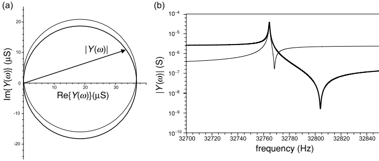
Figure 7.9 Plots of the admittance Y(\omega) . (a) Nyquist plot of the admittance in the complex plane. The values used for the plot are C_0 = 1.2 pF, L = 8.1365 kH, R = 27.1 k \Omega , and C = 2.9 fF. For the thin curve the stray capacitance was increased by a factor of 10. (b) Absolute value of the admittance as a function of the frequency.
