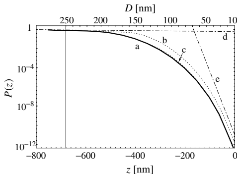
Figure 6.13 Power decay in an infinitely coated aperture probe as a function of distance from the aperture z and of the core diameter D . a: Computed decay, b: mode matching approximation with z_0 = -600 nm, c: mode matching approximation with z_0 = -400 nm, d: decay of the \text{HE}_{11} mode in the cylindrical part of the probe, e: decay of a wave inside bulk aluminum. The vertical line indicates the transition from the cylindrical to the tapered part of the probe.
