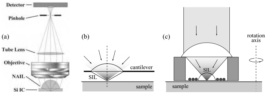
Figure 5.9 SIL technology in three different instruments. (a) Numerical aperture increasing lens microscopy with SIL in contact with sample, (b) SIL microscopy using AFM cantilever for distance control, (c) flying head configuration based on rotating sample surface for magneto-optical data storage.
