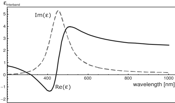
Figure 12.2 Contribution of bound electrons to the dielectric function of gold. The parameters used are \tilde{\omega}_p = 45 \times 10^{14} \text{ s}^{-1} , \gamma = 9 \times 10^{14} \text{ s}^{-1} , and \omega_0 = 2\pi c/\lambda , with \lambda = 450 \text{ nm} . The solid line is the real part, the dashed curve is the imaginary part of the dielectric function associated with bound electrons.
