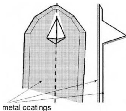
Figure 6.30 Top and side view of an n-doped silicon cantilever with tip. Two successive metal evaporation processes create a Schottky diode at the tip apex. From [55].
