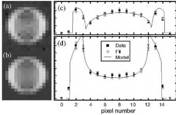
Figure 10.8 Radiation pattern of a single molecule located near a glass surface. The pattern reflects the photons emitted into the dielectric and imaged onto a CCD with a NA = 1.4 objective lens. (a) Data, (b) fitted pattern using Eq. (10.43), (c, d) cross-sections along a horizontal and a vertical line through the center of the pattern, respectively. From [22].
