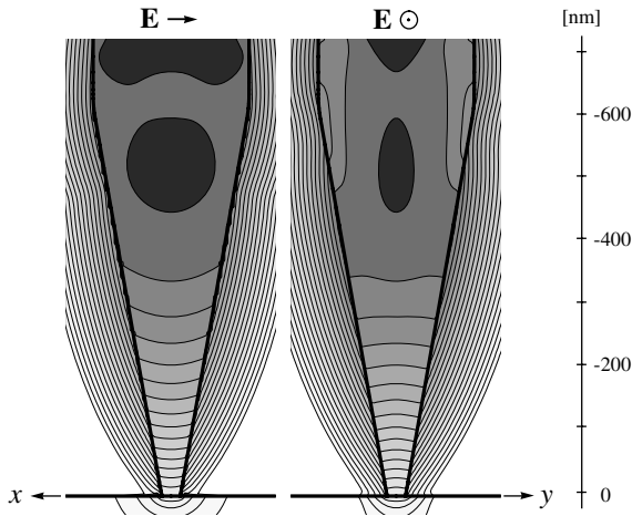
Figure 6.11 Contours of constant power density on two perpendicular planes through the center of an infinitely coated aperture probe (factor of 3 between adjacent lines). The field is excited by the \text{HE}_{11} mode incident from the cylindrical part.
