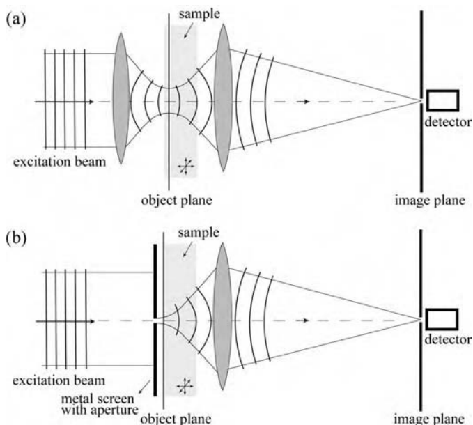
Figure 4.17 Near-field optical microscopy viewed as a generalization of confocal microscopy. (a) In a far-field microscope the propagating field components are focused onto the object plane in the sample. The bandwidth of spatial frequencies is limited to k_{\parallel} < k , where k = n2\pi/\lambda , which sets a limit for the maximum achievable resolution. (b) In a near-field optical microscope the focusing lens is replaced by an object (aperture) which extends the bandwidth of spatial frequencies beyond k . Because the field components with spatial frequencies beyond k do not propagate, the object has to be placed close to the sample.
