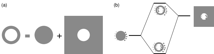
Figure 12.21 Generation of multi-featured surface plasmon resonances by hybridization of elementary modes for the example of a gold nanoshell [37]. (a) Elementary structures. (b) Energies of elementary and hybridized modes.
