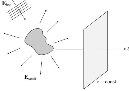
Figure 2.9 In the angular spectrum representation the fields are evaluated in planes ( z = \text{const.} ) perpendicular to an arbitrarily chosen axis z .
