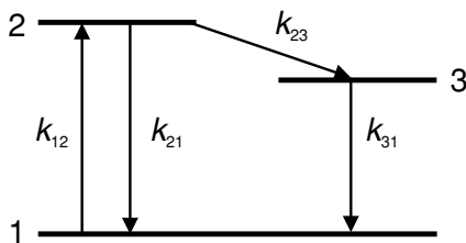
Figure 9.9 A quantum system approximated by a system of three levels. A third level is taken into account in order to accommodate transitions to triplet or dark states.
