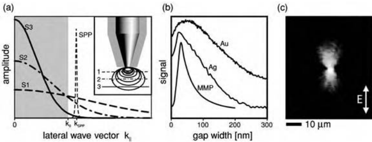
Figure 12.12 Local excitation of surface plasmons with a near-field aperture probe. (a) Sketch of the overlap of the spatial spectra of source (evaluated in planes at different distances from the source) and the surface plasmon on a silver film. (b) Distance dependence of the coupling. The dip at short distances is a result of probe–sample coupling, i.e. the presence of the probe locally modifies the plasmon resonance condition. (c) Image of plasmon propagation recorded by focusing the leakage radiation on an image plane.
