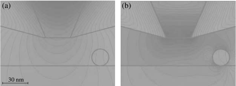
Figure 15.4 Contours of constant |\mathbf{E}|^2 for the model of Fig. 15.3 (log scale, factor of \sqrt{2} between successive lines). (a) s-polarization and (b) p-polarization.
