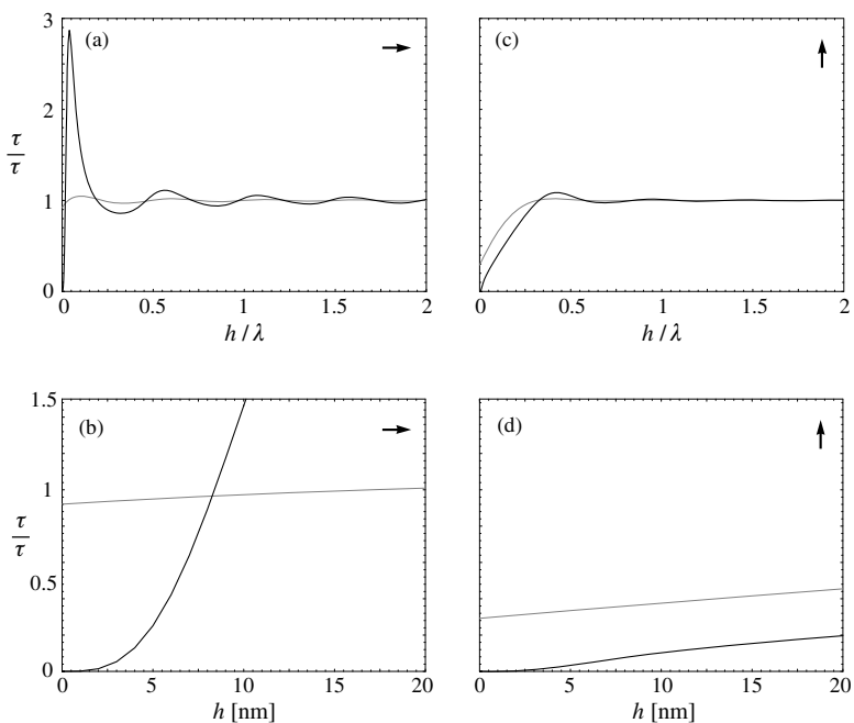
Figure 10.5 Molecular lifetime as a function of the gap h . The dark curves were obtained for an approaching metal interface whereas the bright curves refer to an approaching dielectric interface. The arrows indicate the orientation of the dipole axes. The lower figures are close-ups of the upper ones. The normalization with \tau_0 corresponds to h \rightarrow \infty .
