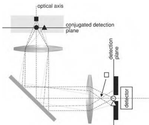
Figure 5.2 Confocal principle. The detection path of a scanning confocal optical microscope is shown. Three objects in the sample are depicted. Only the object (circle) on the optical axis lying in the conjugated detection plane in the object space is imaged onto the pinhole and can be detected. The other objects (triangle and square) are either focused to the side of the pinhole (triangle) or arrive at the pinhole unfocused such that their signals are suppressed.
