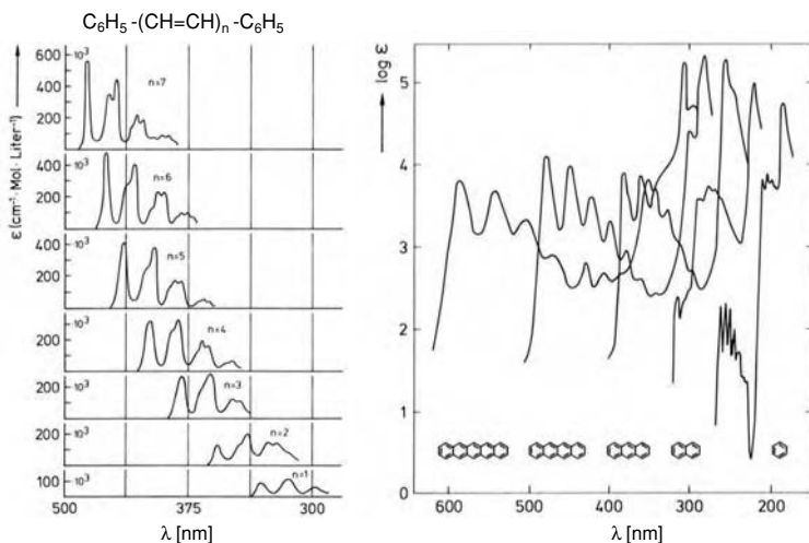
Figure 9.2 Characteristic absorption spectra of fluorescent molecules. Left: Linear polyenes featuring a conjugated carbon chain on which delocalized electrons exist. Right: aromatic molecules. Electrons are delocalized over the aromatic system. Increasing the length of the conjugated chain or the aromatic system shifts the absorption to the red spectral region. From [5].
