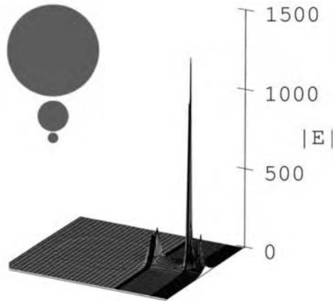
Figure 12.23 Self-similar chain of silver nanoparticles. A very strong resonance is observed for an excitation wavelength of \lambda = 381.5 nm. The associated field enhancement in the gap between the two smallest spheres is larger than 1000. From [45].
