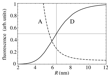
Figure 8.13 Fluorescence intensity of donor and acceptor as a function of their separation R . The donor emission drops to one-half at the distance R = R_0 . The acceptor fluorescence increases as R^{-6} and saturates at a value determined by the acceptor's excited state lifetime.
