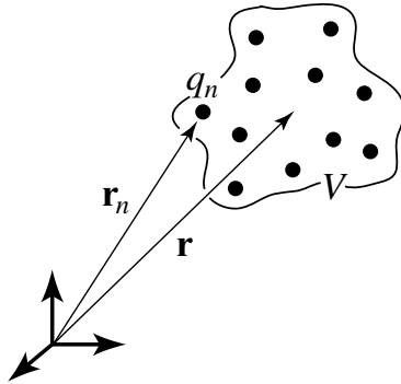
Figure 8.1 In the microscopic picture, optical radiation interacts with the discrete charges q_n of matter. The collective response of the charges with coordinates \mathbf{r}_n can be described by a multipole expansion with origin \mathbf{r} .
