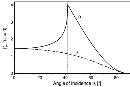
Figure 2.6 Intensity enhancement on top of a glass surface irradiated by a plane wave with variable angle of incidence \theta_i . For a p-polarized wave, the enhancement peaks at the critical angle \theta_c = 41.8^\circ marked by the vertical line.
