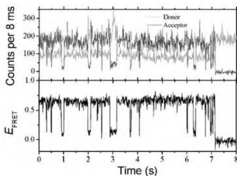
Figure 8.14 Time trajectory of donor and acceptor fluorescence and corresponding FRET efficiency for a donor–acceptor pair attached to a four-way DNA (Holliday) junction. The data indicate that the DNA structure is switching back and forth between two conformations. From [33].
