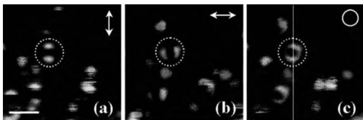
Figure 9.18 Series of three successive fluorescence maps of the same area ( 1.2 \times 1.2 \mu\text{m} ) of a sample of single \text{DiIC}_{18} molecules embedded in a 10 nm thin film of PMMA, measured with the 70 nm aperture probe of Fig. 9.17. The excitation polarization (as measured in the far-field) was changed between linear in the vertical image direction (a), linear in the horizontal image direction (b), and circular (c). The changing polarization affects the molecule's fluorescence rate pattern. For example, for the molecule in the dashed circle it is oriented perpendicular to the sample plane, i.e. pointing in the direction of the near-field probe. Bar = 300 nm. From [27].
