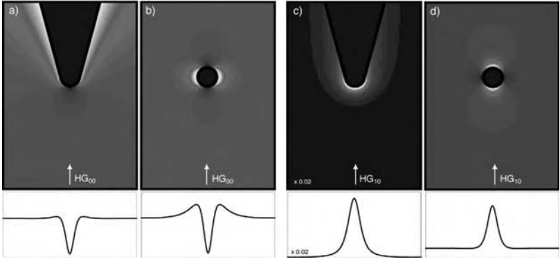
Figure 6.34 Comparison of the near-fields of a metal tip and a metal sphere. (a, b) Excitation with an on-axis, focused ( \text{NA} = 1.4 ) Gaussian beam. (c, d) Excitation with an on-axis, focused Hermite–Gaussian (1, 0) beam. The strong field enhancement in (c) is due to the longitudinal field of the excitation beam. The cross-sections are evaluated in a plane 1 nm beneath the tip. The results indicate that the field distribution near the tip is well approximated by the dipole fields of a small sphere. However, the field strength for longitudinal excitation (c) is much stronger compared with the field strength of an irradiated sphere (d). While in (a, b) the fields are in-phase, they are 155^\circ out of phase in (c, d).
