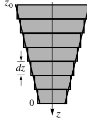
Figure 6.12 Mode matching approximation for the power P(z) in the aperture probe. In each waveguide section the attenuation of the HE_{11} mode is calculated analytically. The contributions of all sections are added and the limit dz \rightarrow 0 is applied.
