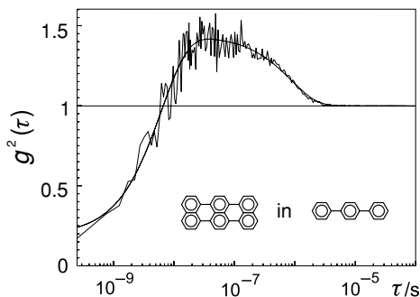
Figure 9.13 Experimentally obtained second-order autocorrelation function g^2(\tau) of a single molecule (terrylene in p -terphenyl). Both antibunching and bunching behavior can be observed. The former occurs at short times whereas the latter is observed for intermediate times at which triplet state excursions are significant. Adapted from [22].
