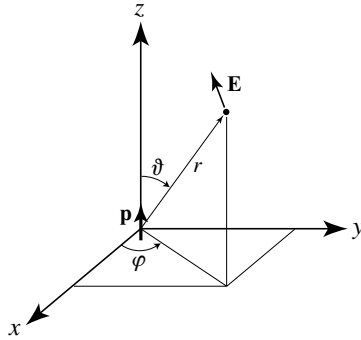
Figure 8.2 The fields of a dipole are most conveniently represented in a spherical coordinate system (r, \vartheta, \varphi) in which the dipole points along the z -axis ( \vartheta = 0 ).
