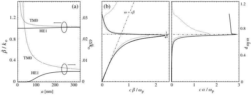
Figure 12.18 (a) Propagation constant k_z = \beta + i\alpha of the two lowest surface modes supported by an aluminum wire at a wavelength of \lambda = 488 nm. a denotes the wire diameter and k_0 = \omega/c . (b) Frequency dispersion of the HE1 surface mode of an a = 50 nm aluminum wire. \omega_p denotes the plasma frequency of aluminum. The dotted line indicates the corresponding dispersion on a plane interface. Notice the backbending effect discussed earlier.
