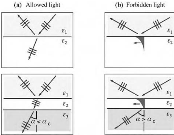
Figure 10.2 Illustration of allowed and forbidden light. The three media fulfill \varepsilon_3 > \varepsilon_1 > \varepsilon_2 . The incident wave hits the upper interface in such a way that (a) a transmitted wave exists and (b) the wave is totally reflected.
