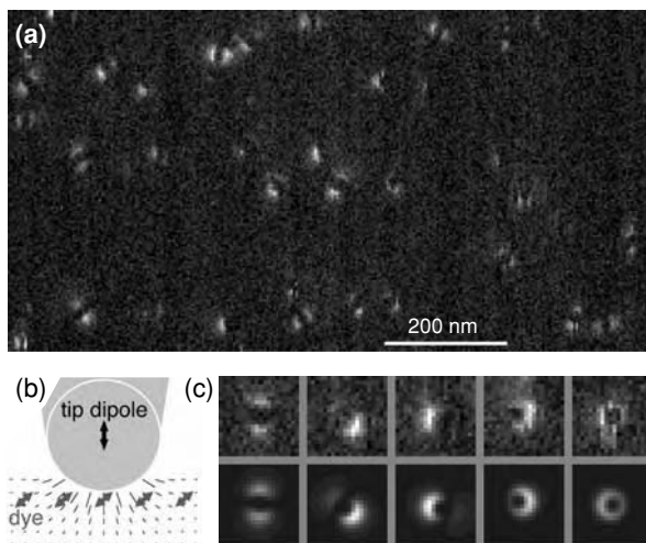
Figure 9.19 Localized field near a sharp metal tip. (a) Fluorescence rate patterns of single molecules scanned by a tip-on-aperture probe. (b) Cut through the rotationally symmetric field distribution near a TAO-probe sampled at different points by a single fluorescent molecule with an out-of-plane orientation of the absorption dipole moment indicated by the arrows. (c) Comparison of theory with selected experimental patterns (see text). From [28].
