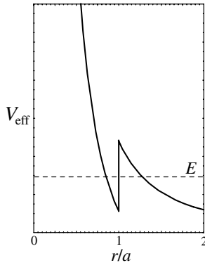
Figure 11.6 Effective potential V_{\text{eff}} for a dielectric sphere according to Eq. (11.30). The radiative decay of a resonant mode can be associated with energy tunneling through the potential barrier. The following parameters were used: \varepsilon_1=2.31 , \varepsilon_2=1 , \lambda=800 nm, l=500 , and a=50 \mu\text{m} .
