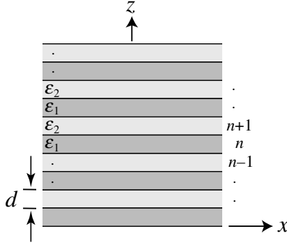
Figure 11.2 One-dimensional photonic crystal made of an infinite number of planar layers of thickness d .
