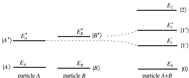
Figure 8.15 Coherent interaction between two particles A and B . In the resonant limit, the excitation becomes delocalized over the two particles.
