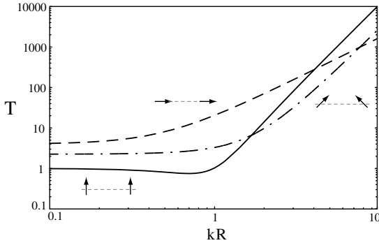
Figure 8.11 Dependence of the function T(\omega) on the distance R between donor and acceptor for different dipole orientations. In all cases, the short distance behavior ( kR \ll 1 ) is constant. Therefore the short distance transfer rate \gamma_{D \rightarrow A} scales as R^{-6} . The long distance behavior ( kR \gg 1 ) depends on the relative orientation of donor and acceptor. If the dipoles are aligned, T(\omega) scales as (kR)^2 and \gamma_{D \rightarrow A} decays as R^{-4} . In all other cases, the long distance behavior of T(\omega) shows a (kR)^4 dependence and \gamma_{D \rightarrow A} decays as (kR)^{-2} .
