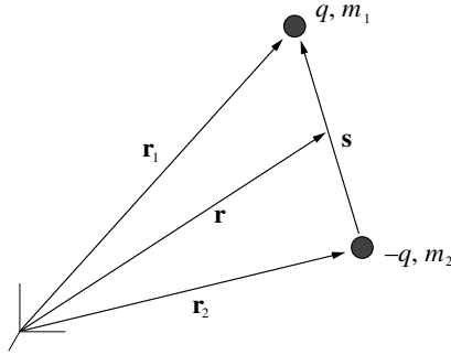
Figure 13.3 Graphical representation of the symbols used to derive the mechanical force in the dipolar limit. \mathbf{r} denotes the center of mass coordinate. The two particles are bound to each other by the potential U .
