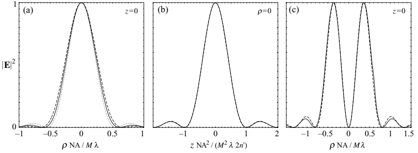
Figure 4.2 (a) Point-spread function depicted in the image plane ( z = 0 ) of a dipole with moment \boldsymbol{\mu} = \mu_x \mathbf{n}_x . The solid curve is the paraxial approximation whereas the dashed and dotted curves are the results of exact calculations for a NA = 1.4 ( n = 1.518 ) objective lens. The dashed curve has been evaluated along the x -axis and the dotted curve along the y -axis. (b) Point-spread function evaluated along the optical axis z . The solid curve is the paraxial approximation and the dashed curve is the exact result for NA = 1.4. (c) Point-spread function depicted in the image plane of a dipole with moment \boldsymbol{\mu} = \mu_z \mathbf{n}_z . The solid curve is the paraxial approximation and the dashed curve is the exact result for NA = 1.4. The figures demonstrate that the paraxial point-spread function is a good approximation even for high NA objective lenses!
