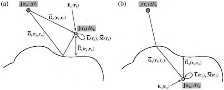
Figure 15.6 Interaction of a volume element \Delta V_k with its environment and with itself. For clarity, only a single interacting volume element \Delta V_n is shown. The arrows indicate the “path” of interaction and the symbols denote the quantities involved. The Green’s function can be split into a primary and a scattering part \vec{\mathbf{G}} = \vec{\mathbf{G}}_0 + \vec{\mathbf{G}}_s and it fulfills the boundary conditions imposed by the reference system.
