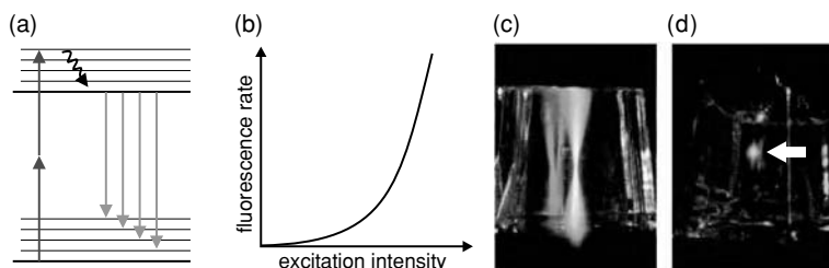
Figure 5.4 Two-photon excitation of a fluorescent molecule. (a) Energy level scheme: A fluorophore with a one-photon absorption in the blue is excited by simultaneous absorption of two near-infrared photons. The emission of the molecule occurs in the green. (b) The fluorescence rate increases as the square of the excitation intensity. This leads to the fact that, while for one-photon excitation the whole beam path in a fluorescent medium lights up (c), for two-photon excitation (d) notable fluorescence is only excited in regions of the highest field strength, e.g. in the focus of a laser beam (see arrow). (c), (d) adapted from [10].
