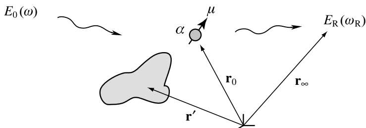
Figure 12.25 General configuration encountered in surface-enhanced spectroscopy. The interaction between a molecule with polarizability \alpha and the exciting field E_0 gives rise to a scattered field E_R . Placing metal nanostructures (coordinate \mathbf{r}' ) near the molecule enhances both the exciting field and the radiated field.
