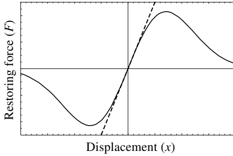
Figure 13.9 Linear approximation (dashed line) to the restoring force (solid line) for a single-beam gradient trap. The slope of the linear approximation is denoted as trap stiffness k . It depends on the particle polarizability, laser power, and field gradients.
