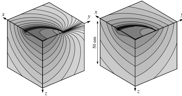
Figure 6.16 Comparison between Bouwkamp's solution (left) and the fields in front of an aperture probe with aluminum coating ( \lambda = 488 nm) calculated by the multiple multipole (MMP) method (right). Contours of constant |\mathbf{E}|^2 (factor of 2 between adjacent lines). The incident polarization is along the x -axis.
