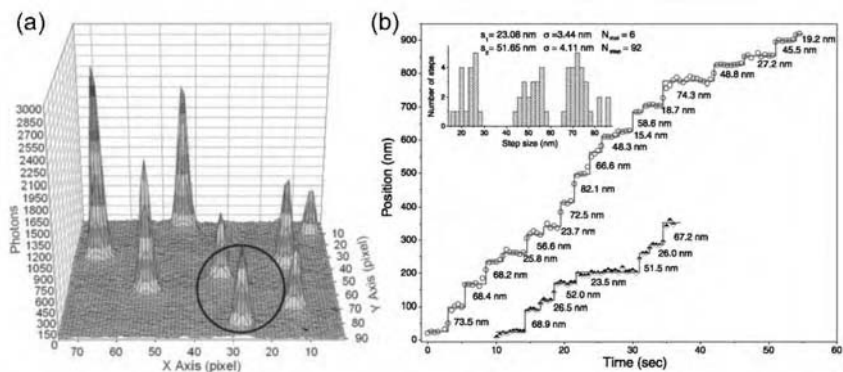
Figure 4.16 Nanometer position accuracy with single dye labels. (a) 3D representation of an image of single Cy3-dyes recorded at an integration time of 0.5 s. Note the high amplitudes of up to 3000 counts and the low background. The variation in amplitude is due to non-uniform illumination. (b) Displacement of individual markers linked to a Myosin V motor protein vs. time. The stepwise motion of the marker is clearly resolved. Adapted from Ref. [17].
