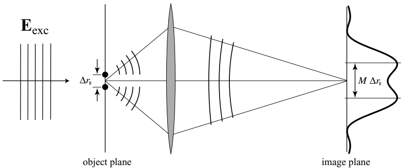
Figure 4.3 Illustration of the resolution limit. Two simultaneously radiating point sources separated by \Delta r_{||} in the object plane generate a combined point-spread function in the image plane. The two point sources are optically resolved if they can be distinguished based on their image pattern.
