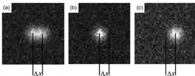
Figure 4.11 Simulated image pattern of two nearby emitters with a constant Poissonian background. The emitters are simulated to exhibit Gaussian patterns with Poissonian noise uncorrelated to the background noise. (a) Two emitters without discrimination of photons. (b), (c) Individual patterns obtained by energy discrimination of photons. The individual patterns are displaced by finite distance \Delta x .
