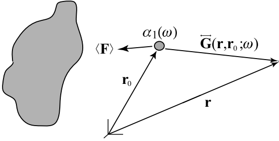
Figure 14.6 Dispersion force acting on a polarizable particle located at \mathbf{r} = \mathbf{r}_0 . The force originates from correlated charge fluctuations in the particle and other bodies in the environment. The latter are accounted for by the Green's function \vec{\vec{G}} evaluated at its origin.
