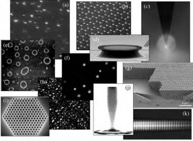
Figure 1.1 Potpourri of man-made nanophotonic structures. (a) Strongly fluorescent molecules, (b) metal nanostructures fabricated by nanosphere lithography, (c) localized photon sources, (d) microdisk resonators (from [2]), (e) semiconductor nanostructures, (f) particle plasmons (from [3]), (g) photonic bandgap crystals (from [4]), (h) nanocomposite materials, (i) laser microcavities (from [5]), (j) single photon sources (from [6]), (k) surface plasmon waveguides (from [7]).
