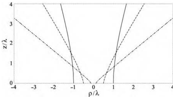
Figure 4.19 Divergence of optical fields with different confinements in the source plane. The same parameters are used as in Fig. 4.18. A point on a line denotes the radial distance for which the field strength of E_x decays to 1/e of its on-axis value. The better the confinement in the source plane at z=0 , the faster the fields will diverge.
