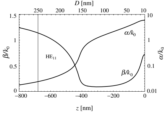
Figure 6.14 Attenuation constant \alpha_{11} and phase constant \beta_{11} of the cylindrical \text{HE}_{11} mode as a function of the core diameter D . z is the corresponding distance from the aperture. The vertical line indicates the transition from the cylindrical to the tapered part of the aperture probe. From [21].
