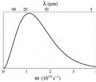
Figure 14.4 Blackbody radiation spectrum \overline{W}_\omega^+ for T = 300 K. Equilibrium conditions require that the net Poynting vector vanishes everywhere.
