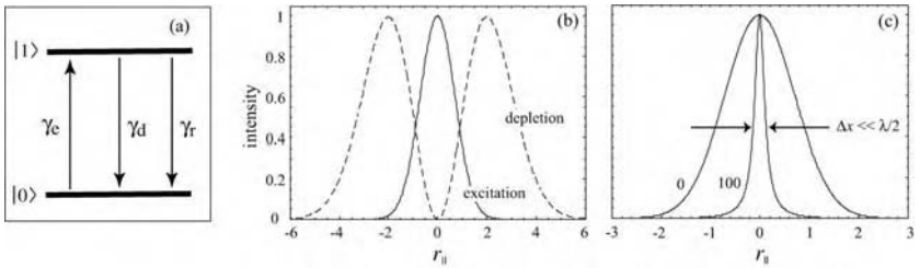
Figure 4.7 Illustration of resolution enhancement through saturation. (a) Energy level diagram of a two-state molecule with excitation rate \gamma_e , radiative decay rate \gamma_r , and stimulated depletion rate \gamma_d . (b) Transverse intensity profiles of excitation field and depletion field. The zero of the depletion field is placed at the maximum of the excitation field. (c) Transverse fluorescence profiles ( \gamma_f ) for two different depletion parameters d_p = 0 and d_p = 100 . The higher d_p the narrower the fluorescence peak will be.
