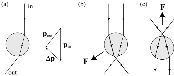
Figure 13.8 Illustration of the ray-optic picture for optical trapping of particles larger than the wavelength. (a) A single ray is refracted twice at the surface of the particle. The net momentum change \Delta \mathbf{p} is calculated by the vectorial difference of the momenta of incoming and outgoing rays. Momentum conservation requires that the momentum transferred to the particle is -\Delta \mathbf{p} . (b) Refraction of two light rays with different intensities. The particle is pulled towards the higher intensity. (c) Axial trapping of a particle in a single-beam trap. A particle initially located beneath the focus is pulled towards the focus.
