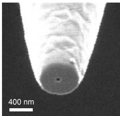
Figure 9.17 Image of a near-field aperture probe of which the end face was cut by focused ion beam milling. The aperture that shows up in the circular facet has a diameter of 70(\pm 5) nm. The probes have flat end faces and the apertures have well-defined edges and are circularly symmetric. From [27].
