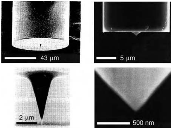
Figure 6.4 Scanning electron microscopy images of fiber tips etched by Ohtsu's method. Left: Highly Ge-doped special fiber. From [6] with permission. Right: Commercial fiber. From [79].
