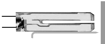
Figure 7.6 Cartoon of a quartz tuning-fork sensor with attached tapered glass fiber (to scale) showing the relative dimensions of fiber probe and tuning-fork sensor. Left: sensor. Right: sample.
