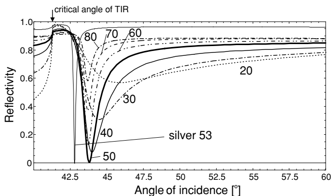
Figure 12.8 Excitation of surface plasmons in the Kretschmann configuration. The reflectivity of the exciting beam is plotted as a function of the incident angle and for different air gaps (in nm). The curves are evaluated for a gold film. For comparison a single trace is also plotted for silver. Note the much sharper resonance due to the smaller damping of silver as compared to gold. The critical angle of total internal reflection shows up as a discontinuity marked by an arrow.
