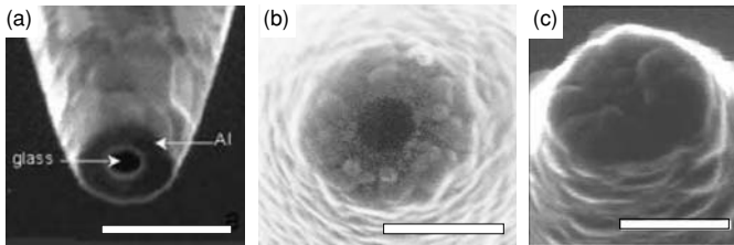
Figure 6.22 Grains and apertures in aluminum-coated optical probes. (a) Image of an aluminum-coated optical probe recorded in a focused ion beam apparatus. The enhanced visibility of grains is caused by ion-channeling effects in grain boundaries (see e.g. [37]). The aperture is well defined because the apex was cut off by the focused ion beam. Image courtesy of N. F. van Hulst (b), (c) Scanning electron microscope image of a pristine aperture with large grains. From [17]. Scale bars are 300 nm.
