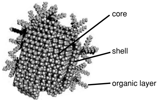
Figure 9.3 Structure of a typical colloidal semiconductor nanocrystal. Courtesy of Hans Eisler.
