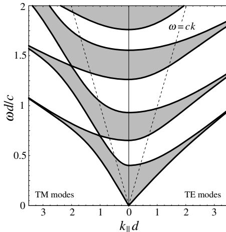
Figure 11.3 Band diagram for a one-dimensional photonic crystal. The shaded areas are the allowed bands. The diagram represents both TE and TM modes. For a 1D photonic crystal, there are no complete bandgaps, i.e. there are no frequencies for which propagation is inhibited in all directions. Values used: \varepsilon_1 = 2.33 ( \text{SiO}_2 ), \varepsilon_2 = 17.88 ( \text{InSb} ).
