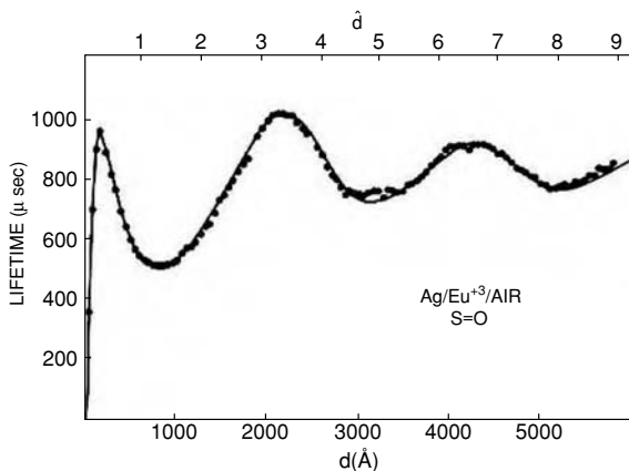
Figure 8.8 Comparison of classical theory and experimental data of molecular lifetimes in inhomogeneous environments. In the experiment, a layer of \text{Eu}^{3+} ions is held by fatty acid spacers of variable thickness close to a silver surface (data after Drexhage [20]). The calculated curve is due to Chance et al. [21].
