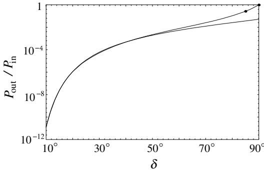
Figure 6.15 Dependence of power transmission on taper angle ( \delta = half-cone angle). The aperture diameter is 20 nm and the wavelength \lambda = 488 nm. Changing the taper angle from 10^\circ to 45^\circ increases the power throughput by nine orders of magnitude. Three-dimensional computation (points) and according to Eq. (6.12) with a value of B = 3.6 (solid line).
