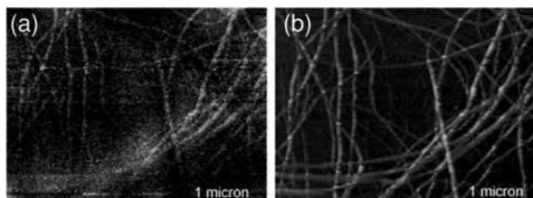
Figure 5.12 Imaging with a tip-enhanced scanning near-field optical microscope using two-photon excitation. (a) Two-photon excited fluorescence of a sample of PIC J-aggregates on glass. (b) Corresponding topographical image recorded with tuning-fork shear-force feedback.
