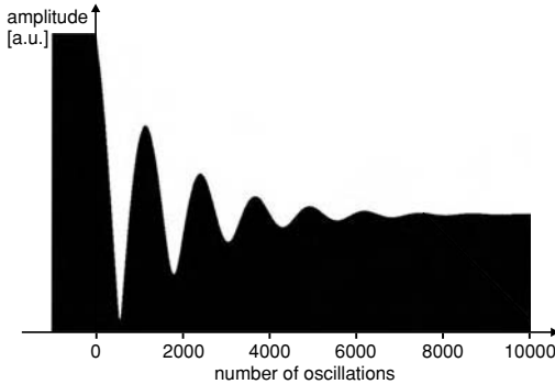
Figure 7.7 Transient response of an oscillating tuning fork ( Q = 2886 ) upon a change in probe-sample distance d at t = 0 . The step causes a resonance frequency shift of 16.5 Hz from 33 000 to 33 016.5 Hz following Eq. (7.16). Only after \sim 2Q = 10\,000 oscillation periods is the new steady state reached. Individual oscillations cannot be resolved – only the envelope is visible.
