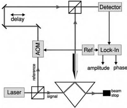
Figure 5.20 Photon tunneling microscopy combined with time-resolved heterodyne interferometry. The light from a fixed-frequency laser source is divided into a reference and a signal branch. In the reference branch the frequency is shifted by means of an acousto-optic modulator (AOM). Furthermore, in the reference branch there is a delay line for time-resolved experiments. The signal branch undergoes total internal reflection inside a prism and provides evanescent field illumination at a structure of interest. An evanescent field can also be created by coupling the signal branch into a waveguide. A sharp fiber probes the evanescent field above the sample and directs the sampled light to a beamsplitter where the sampled light interferes with the reference field. The resulting signal is analyzed with a lock-in amplifier.
