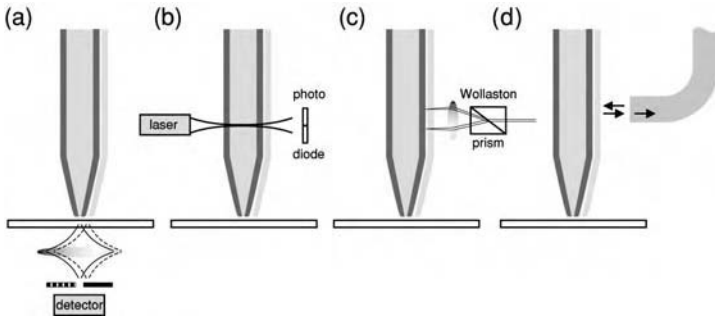
Figure 7.4 Different methods for the direct detection of the oscillation of an optical probe. (a) Aperture detection scheme: the light emitted or scattered by the probe is focused onto a pinhole. The detected light is modulated at the mechanical resonance frequency of the probe. (b) Laser deflection scheme: an infrared diode laser is scattered or deflected by the fiber probe. The resulting oscillating fringe pattern is directed to a split photodiode. (c) Differential interferometry using a Wollaston prism. (d) Interferometry using a fiber optic interferometer.
