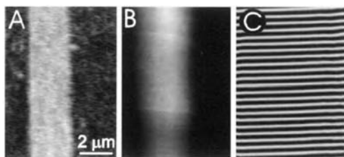
Figure 5.21 Field distribution above a \text{Si}_3\text{N}_4 channel waveguide. Linearly polarized light has been coupled into the channel waveguide to excite only the \text{TM}_{00} mode. (A) Topography recorded with shear-force feedback. (B) Amplitude of the field distribution. (C) Cosine of the measured phase distribution. From [40].
