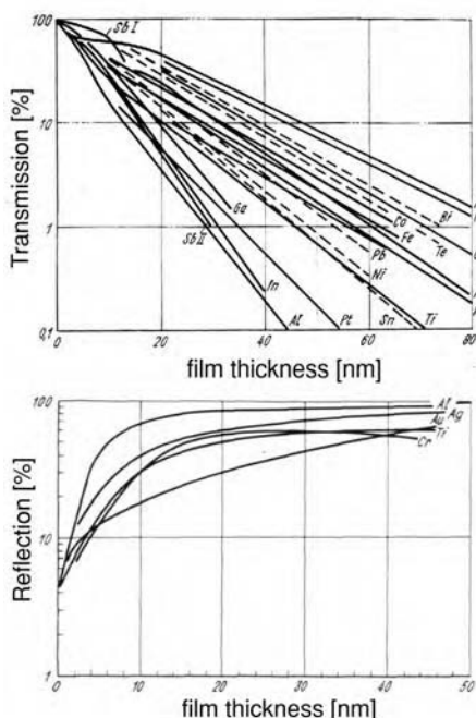
Figure 6.20 Transmission and reflection of thin films as a function of the film thickness for various metals. Measurements were performed at a wavelength of 550 \pm 5 nm for Ag, Au, Cu, Ga, In, Mn, Pd, Al, Co, Cr, Fe, Pt, Ti, and Sb and at a wavelength of 503 \pm 5 nm for Ni, Pb, Sn and using white light for Bi and Te. The films were thermally evaporated at a pressure of 1 \times 10^{-5} Torr at a rate of \approx 100 nm/min and then tempered at a few hundred degrees Celsius in vacuum. From [36].
