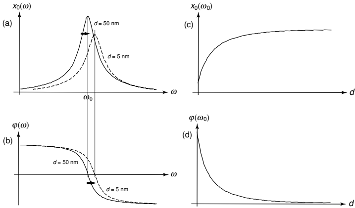
Figure 7.3 Resonance of a vibrating beam. Amplitude (a) and phase (b) of a beam driven at a frequency \omega . As the beam-end starts to interact with a sample surface, the resonance shifts and the amplitude drops. (c, d) show the amplitude and phase at frequency \omega = \omega_0 as a function of the distance between beam-end (tip) and surface. The distance-range over which the amplitude and phase vary depends on the interaction area (tip sharpness).
