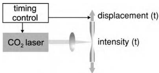
Figure 6.5 Sketch of a typical set-up for pulling of optical fibers using a CO 2 laser. The laser is focused onto the fiber. For heating, a laser pulse of some milliseconds is applied. The pulling starts after the laser pulse and follows a distinct velocity profile. See e.g. [9] for details.
