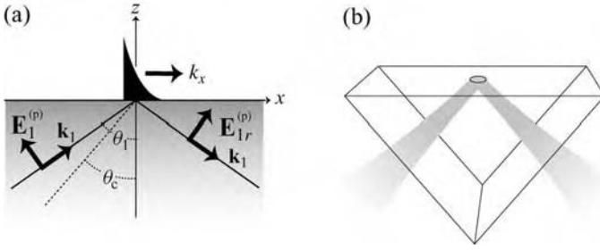
Figure 2.4 Excitation of an evanescent wave by total internal reflection. (a) An evanescent wave is created in a medium if the plane wave is incident at an angle \theta_i > \theta_c . (b) Actual experimental realization using a prism and a weakly focused Gaussian beam.
