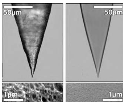
Figure 6.3 Etched fiber tips. Left: Turner's method. Right: Tube-etched tip. The upper panels show optical images taken with a conventional microscope. The lower panel shows higher-resolution scanning electron micrographs of the surface roughness of the tips sputtered with 3 nm platinum at 77 K. From [5].
