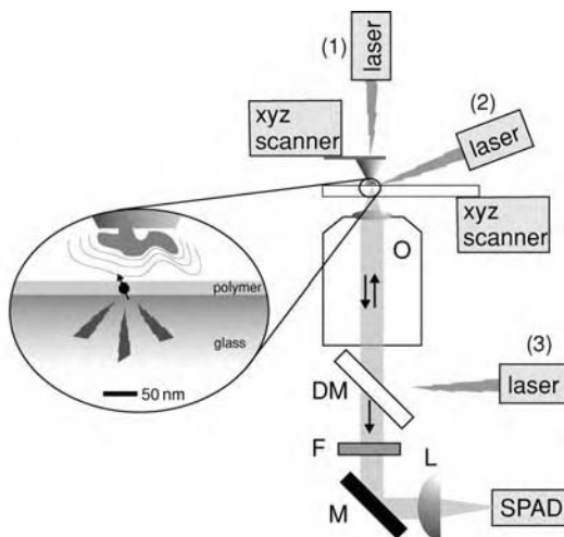
Figure 9.14 Schematic set-up for metrology of confined fields using single fluorescent molecules with different possible illumination geometries (1), (2) and (3).
