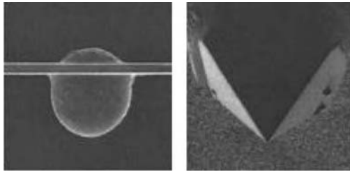
Figure 6.28 AFM cantilever modified by focused ion beam milling. For details see text. From [51].
