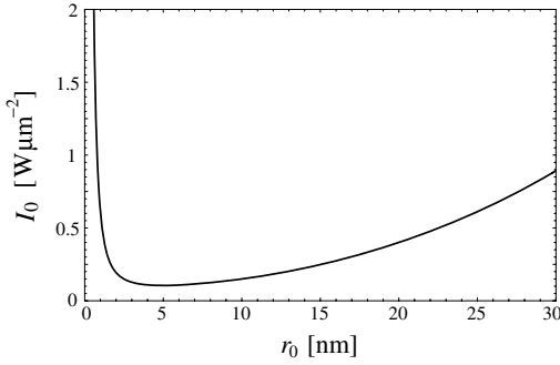
Figure 13.14 Minimum trapping intensity I_0 as a function of the particle radius r_0 . An enhancement factor of f = 3000 is assumed and the tip radius is r_t = 5 nm.
