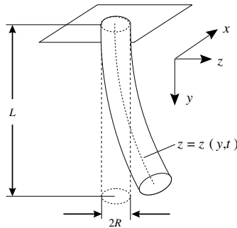
Figure 7.2 Sketch of a quartz beam of length L used to calculate the resonances of an oscillating fiber probe.
