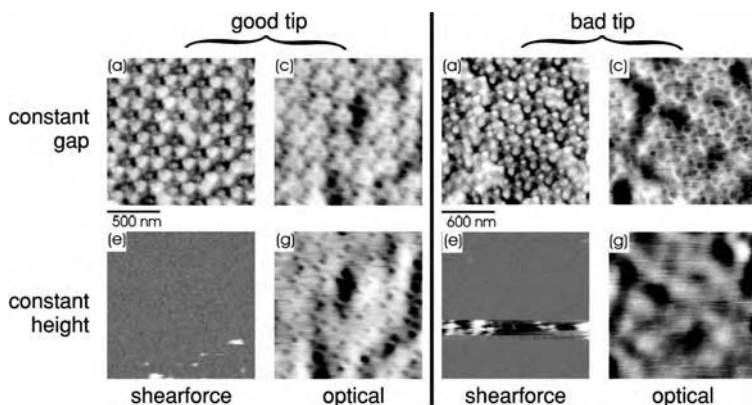
Figure 7.15 Imaging of a latex sphere projection pattern in constant-gap mode (upper row) and constant-height mode (lower row) with two different near-field probes, a “good” probe with an aperture of 50 nm (left side) and a “bad” probe with an aperture of 200 nm (right side). The constant-gap topographic and optical images show sharp features for both probes but only the constant-height mode image for the “good” probe shows optical contrast.
