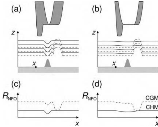
Figure 7.14 Influence of probe geometry on recorded scan images. The near-field signal S_{\text{NFO}} is represented by solid lines and the feedback signal S_{\text{SF}} by dashed lines. Both scan-lines are plotted relative to the center of the aperture probe. The mini-tip on the rim of the aperture is oversized to better visualize the resulting effects. (c, d) Recorded scan-lines for different modes of operation: constant-gap mode (CGM) and constant-height mode (CHM). CGM introduces artifacts because of the varying probe-sample distance. From [3].
