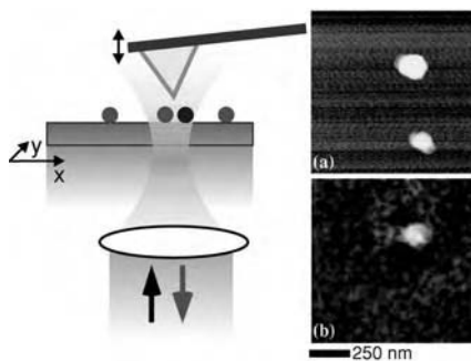
Figure 5.26 Imaging of 60 nm fluorescent beads based on local quenching with a gold-coated AFM tip. The left panel shows a scheme of the experimental arrangement. It combines a tapping-mode AFM with an inverted optical microscope. The optical signal is created by gated photon counting. The count rate at the closest contact to the sample was subtracted from the count rate at the upper turning point of the tapping cantilever. This yields a positive signal if the count rate is reduced at close contact between tip and sample, e.g. due to quenching. (a) Tapping mode AFM topographic image of a 60 nm fluorescent bead and a contaminating particle. (b) Only the bead is visible in the optical image. Adapted from [34].
