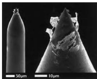
Figure 6.23 Destruction of an aperture probe by excessive input of light. From [20].
