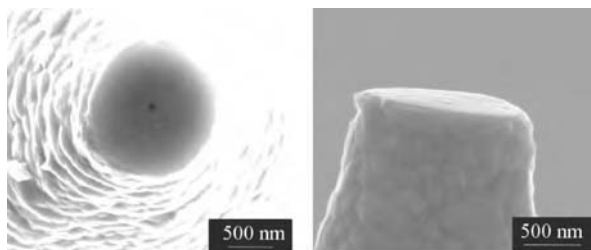
Figure 6.24 Aperture at the apex of an optical probe created using the CASSE technique [43]. Note the small diameter of the aperture (dark region in the center) and the smooth endface. Image courtesy of J. Toquand and D. W. Pohl.
