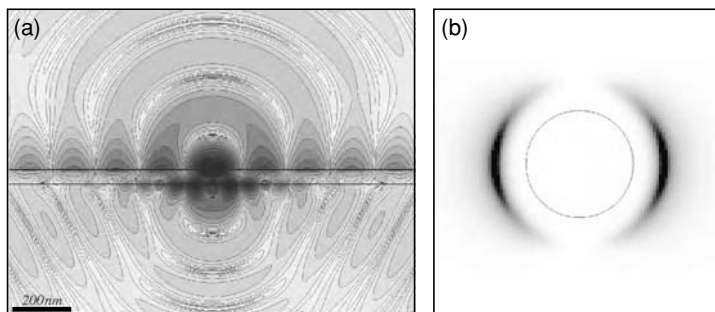
Figure 12.11 Excitation of surface plasmons with a dipole source placed 5 nm above a 50 nm silver layer supported by a glass substrate. The excitation wavelength is 370 nm and the dipole moment is parallel to the interface. (a) Lines of constant power density (factor of 2 between successive contour lines) depicted at a certain instant of time. The figure shows the surface plasmon propagation along the top surface of the silver film and also the radiative decay into the lower half-space. (b) Radiation pattern evaluated on a horizontal plane in the lower medium. The circle indicates the critical angle of total internal reflection at an air/glass interface. The two lobes result from the radiative decay of surface plasmons excited by the dipole source.
