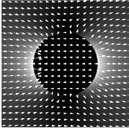
Figure 12.17 Near-field distribution around a gold wire in the quasi-static limit \varepsilon_1 = -18 , \varepsilon_2 = 2.25 . Grayscale: |E|^2 ; arrows: direction and magnitude of the electric field.
