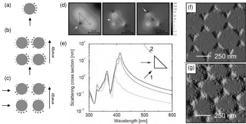
Figure 12.22 Shape effects in particle-plasmon resonances. (a) Elementary mode of a spherical particle. The arrow indicates the direction of incidence of the exciting field. (b), (c) Surface charge distributions of hybrid plasmon modes associated with particle pairs (qualitative). The direction of incidence is perpendicular (b) and parallel (c) to the long axis of the particle. (d) Near-field distribution of resonant silver nanowires with triangular cross-sections. The direction of incidence is indicated by white arrows. (e) Scattering spectra corresponding to the distributions shown in (d). From [38]. (f) and (g) show AFM images of triangular resonant silver particles created by nanosphere lithography used for the detection of Alzheimer’s disease. (f) is without attached antibodies and (g) is with attached antibodies. From [39].
