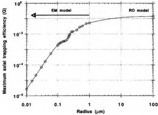
Figure 13.7 Calculated maximum axial trapping efficiency \text{Max}[Q_z(x = 0, y = 0, z)] for a polystyrene particle ( \epsilon = 2.46 ) with variable radius r_0 irradiated by a focused Gaussian beam. The surrounding medium is water ( \epsilon_s = 1.77 ) and the numerical aperture is 1.15. From [10].
