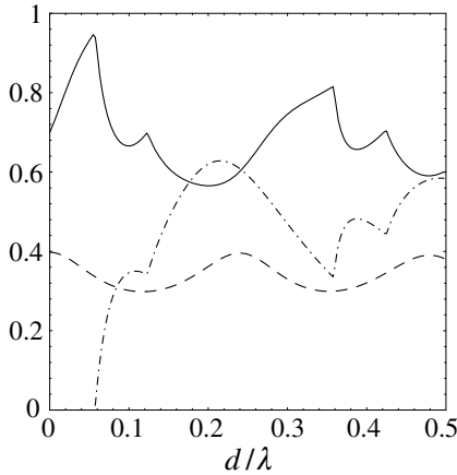
Figure 10.10 Allowed light ( P_a^\downarrow , dashed curve), forbidden light ( P_f^\downarrow , solid curve) and radiation coupled into the waveguide ( P_m = P - P^\uparrow - P^\downarrow , dash-dotted curve) as a function of the thickness d of the slab waveguide characterized in Fig. 10.3. The discontinuities correspond to the cut-offs of the TE_0 , TM_0 , TE_1 and TM_1 modes.
