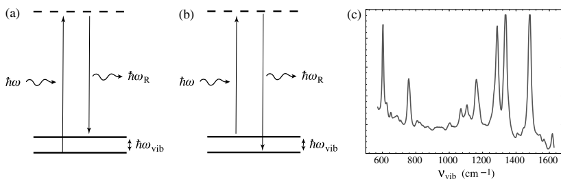
Figure 12.24 Raman scattering refers to the spectroscopic process in which a molecule absorbs a photon with frequency \omega and subsequently emits a photon at a different frequency \omega_R , which is offset with respect to \omega by a vibrational frequency \omega_{\text{vib}} of the molecule, i.e. \omega_R = \omega \pm \omega_{\text{vib}} . Absorption and emission are mediated by a virtual state, i.e. a vacuum state that does not match any molecular energy level. (a) If \omega > \omega_R , one speaks of Stokes Raman scattering, and (b) if \omega < \omega_R , the process is designated as anti-Stokes Raman scattering. (c) Raman scattering spectrum representing the vibrational frequencies of Rhodamine 6G. The spectrum is expressed in wavenumbers \nu_{\text{vib}}(\text{cm}^{-1}) = [1/\lambda(\text{cm})] - [1/\lambda_R(\text{cm})] , with \lambda and \lambda_R being the wavelengths of incident and scattered light, respectively.
