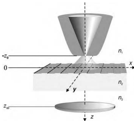
Figure 4.20 Mapping of information from a sample plane ( z = 0 ) to a detector plane ( z = z_{\infty} \gg \lambda ) using a confined source field at z = -z_0 . The high spatial frequencies of the sample can be detected by using a strongly confined source field in close proximity to the sample ( z_0 \ll \lambda ). In scanning near-field optical microscopy, the detector field is usually focused onto a point detector.
