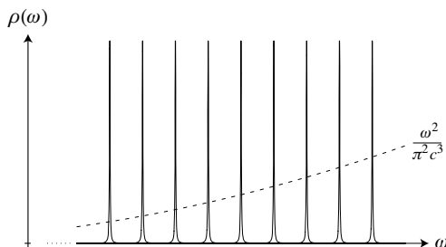
Figure 11.9 Photonic density of states of a microsphere (solid line) and in free space (dashed line). In a microsphere all energy is concentrated in the narrow frequency windows of individual resonant modes.
