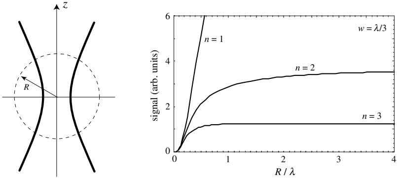
Figure 4.10 Localization of the excitation volume in multiphoton microscopy. The figure depicts the signal that is generated in a dense sample within a sphere of radius R when excited by a focused Gaussian beam by n -photon excitation. Different from multiphoton excitation ( n > 1 ), one-photon excitation ( n = 1 ) cannot restrict the excitation volume without the use of a confocal pinhole.
