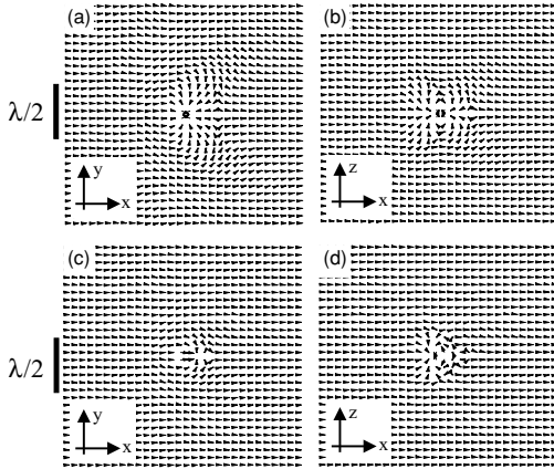
Figure 9.8 Time-averaged Poynting vector (excitation and extinction part) in a 2 \times 2 \lambda area around a dipole oscillating in the z -direction excited by a plane wave polarized in the z -direction and propagating in the x -direction. (a), (b) depict the (x, y) and (x, z) planes, respectively, for zero detuning. (c), (d) show the (x, y) and (x, z) planes, respectively, for a detuning of one linewidth. The energy flow is directed towards the point dipole over a large area and even comes back to the dipole after it has already passed by. Out of resonance the effective area decreases markedly (c), (d).
