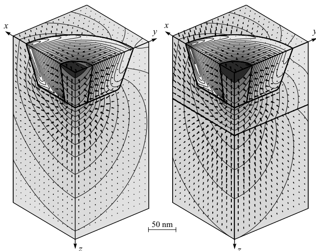
Figure 6.17 Contours of constant |E|^2 on three perpendicular planes near the fore-most end of an aperture probe (factor of 2 between successive lines). The arrows indicate the time averaged Poynting vector. The incident polarization is in the plane y = 0 . The transmission through the probe is increased when a dielectric substrate ( \epsilon = 2.25 ) is brought close (right figure).
