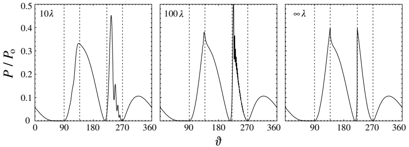
Figure 10.9 Angular distribution of power radiated from a dipole with orientation \theta = 60^\circ and height h = 20 nm above a dielectric half-space. \lambda = 633 nm, \varepsilon_1 = 1 , \varepsilon_2 = 2.25 . The radiation patterns are shown for different distances from the dipole's origin and are depicted in the (x, z) -plane. The lower half-space corresponds to 90^\circ < \theta < 270^\circ . The interface and the critical angle are shown as dashed vertical lines.
