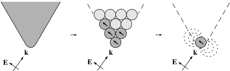
Figure 13.6 Illustration of the coupled dipole approach. A macroscopic object is subdivided into individual microscopic dipolar subunits. Each dipole moment can be calculated self-consistently by using the Green's function formalism. In a rough approximation the field in front of a metal tip can be replaced by the field of a single dipole. However, the parameters of the polarizability have to be deduced from a rigorous calculation.
