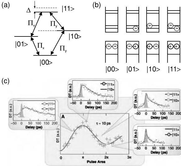
Figure 9.7 Coherent control of the state of a biexciton. (a) Energy level scheme. (b) Corresponding exciton transitions encoding two qubits. (c) Biexciton Rabi oscillation demonstrating the possibility to realize a controlled rotation quantum logic gate using the biexciton transitions shown in (a). Adapted from [16].
