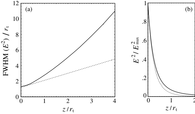
Figure 13.12 Comparison of the non-retarded fields of a single dipole (dotted curves) and the computationally determined fields for a laser-illuminated metal tip (solid curves). (a) The lateral spread of the field (perpendicular to tip axis) as a function of the distance z from the foremost point of the tip. (b) The decay of the field along the tip axis. All distances are normalized with the tip radius r_t = 5 nm.
