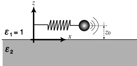
Figure 14.8 A particle in vacuum moves parallel to a planar substrate with a dielectric function \varepsilon_2(\omega) .
