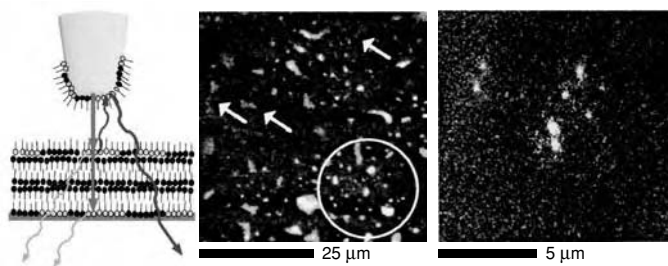
Figure 5.28 Near-field microscopy based on fluorescence resonance energy transfer (FRET). Left: Cartoon of the experiment. The donor molecules are located in a multilayer Langmuir–Blodgett (LB) film whereas the acceptor molecules are supported by a LB layer deposited on a tip. The donor fluoresces in the green if the tip is absent. On the other hand, additional red fluorescence is observed in the presence of the tip because of FRET between the topmost layer of the LB film and the tip. Middle: FRET image of a 50 \times 50 \mu\text{m} area of the sample. Patches of fluorescence are observed revealing donor islands in the LB film. Right: Spatial resolution achieved in these experiments. Adapted from [52].
