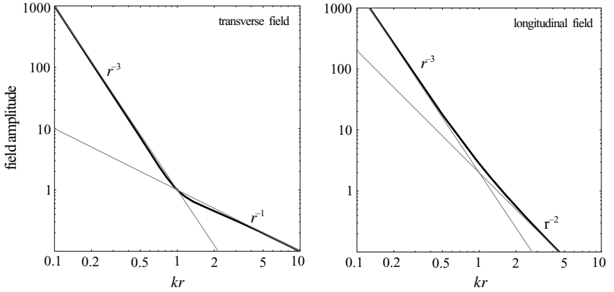
Figure 8.3 Radial decay of the dipole's transverse and longitudinal fields. The curves correspond to the absolute value of the expressions in brackets of Eqs. (8.62) and (8.63), respectively. While both the transverse and the longitudinal field contribute to the near-field, only the transverse field survives in the far-field. Notice that the intermediate-field with (kr)^{-2} does not really show up for the transverse field. Instead the near-field dominates for (kr) < 1 and the far-field for (kr) > 1 .
