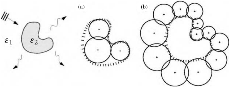
Figure 15.2 MMP modeling of a single scatterer. (a) Multipoles for the outer domain, (b) multipoles for the inner domain. The circles indicate the area of greatest influence. The boundary is discretized and to each matching point the normal vector is indicated.
