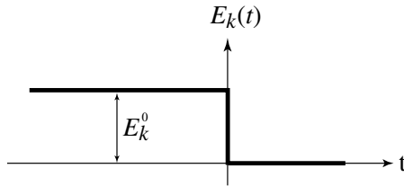
Figure 14.2 Time dependence of the considered perturbation. The perturbation ensures complete relaxation of the system at times t = 0 (immediately before the step) and t \rightarrow \infty .
