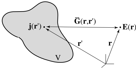
Figure 2.3 Illustration of the dyadic Green's function \vec{\mathbf{G}}(\mathbf{r}, \mathbf{r}') . The Green's function renders the electric field at the field point \mathbf{r} due to a single point source \mathbf{j} at the source point \mathbf{r}' . Since the field at \mathbf{r} depends on the orientation of \mathbf{j} the Green's function must account for all possible orientations in the form of a tensor.
