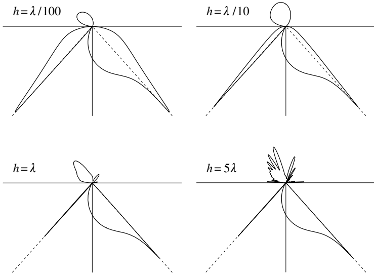
Figure 10.7 Radiation patterns of a dipole with orientation \theta = 60^\circ approaching a planar waveguide. \lambda = 488 nm, \delta = 80 nm, \varepsilon_1 = 1 , \varepsilon_2 = 5 , \varepsilon_3 = 2.25 . The different heights z_0 = h of the dipole are indicated in the figure. The radiation patterns are shown in the plane defined by the dipole axis and the z -axis. Note that the allowed light does not depend on h and that the forbidden light is always symmetrical with respect to the vertical axis.
