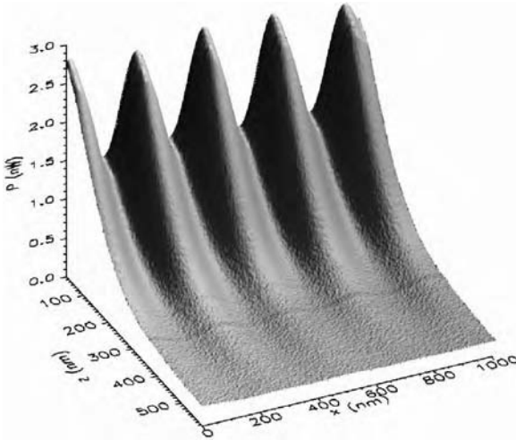
Figure 2.5 Spatial modulation of the standing evanescent wave along the propagation direction of two interfering waves ( x -axis) and the decay of the intensity in the z -direction. The ordinate represents the measured optical power. From [9].
