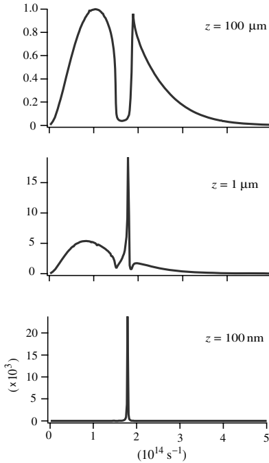
Figure 14.5 Spectra of thermal emission from a semi-infinite sample of SiC at T = 300 K evaluated at three different heights z above the surface. From [7].
