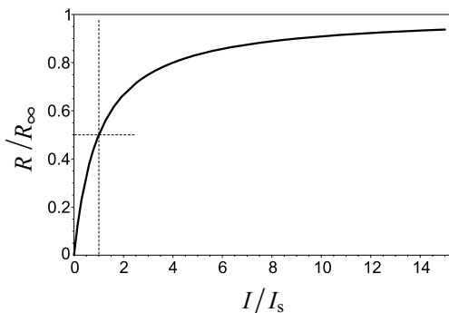
Figure 9.10 Saturation of the emission rate of a single molecule as a function of the excitation intensity.
