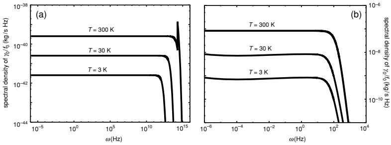
Figure 14.9 Normalized spectral density of the damping coefficient as a function of the angular frequency \omega for temperatures T = 3 K, 30 K, 300 K. f_0 = a^3/z_0^5 , where a (particle radius) and z_0 (tip-sample distance) are defined in nanometers. (a) Substrate and particle made of a metal (Ag); (b) substrate and particle made of a dielectric ( \text{SiO}_2 ). From [17].
