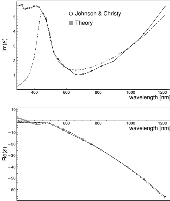
Figure 12.3 Dielectric function of gold: Experimental values and model. Upper panel: Imaginary part. Lower panel: Real part. Open circles: Experimental values taken from [6]. Squares: Model of the dielectric function taking into account the free-electron contribution and the contribution of a single interband transition. Note the different scales for the abscissae.
