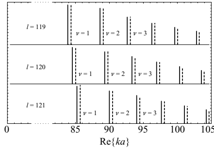
Figure 11.8 Normalized mode frequencies for a microsphere with \varepsilon = 2.31 and angular momentum mode numbers l = 119 , l = 120 , and l = 121 . Solid lines are TE modes and dashed lines are TM modes. The height of the lines indicates the quality factor on a logarithmic scale. The \nu = 1 modes have a Q-factor of \approx 10^{17} and the \nu = 6 modes of \approx 10^6 .
