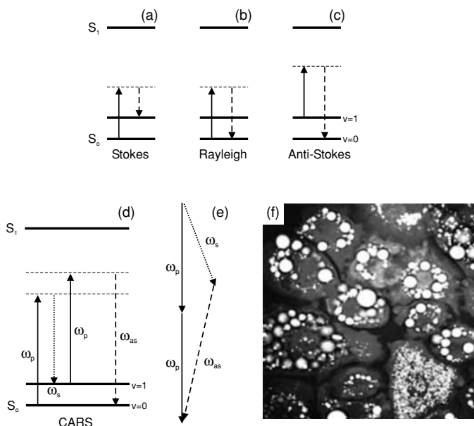
Figure 5.6 Energy diagram of spontaneous Raman scattering and coherent anti-Stokes Raman scattering (CARS). Light scattering from a molecule can result in (a) Stokes-shifted photons, (b) Rayleigh scattering, or (c) anti-Stokes emission (d). CARS is a four-wave mixing process using two tunable (pulsed) lasers at \omega_p and \omega_s . If the difference in frequency between the two lasers hits the energy of a vibration, the CARS signal \omega_{as} is enhanced and emitted preferentially into a direction determined by the phase matching condition (e). (f) An image of fibroblast cells stimulated to produce lipids. The lipid droplets can be visualized using CARS when tuning to the aliphatic C-H vibration. The 100 \times 100 \mu\text{m}^2 image was taken in 2.7 s. Image courtesy of X. S. Xie, Harvard University.
