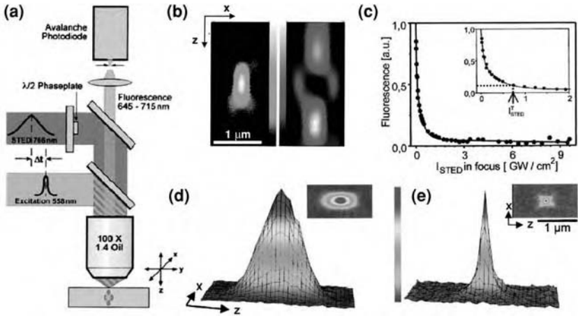
Figure 5.5 Principle of stimulated emission depletion confocal microscopy. (a) Set-up of the STED confocal microscope. A short excitation pulse and a long depletion pulse are coupled into a microscope objective. The depletion beam is engineered so that it shows zero intensity at the geometrical focus (b, right panel) while the excitation beam shows the usual focus (b, left panel). (c) Fluorescence from the confocal volume as a function of the depletion beam intensity. Note the strongly nonlinear behavior. (d) Point-spread function without and with depletion beam switched on (e). Adapted from [11].
