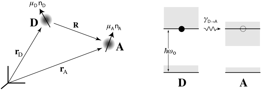
Figure 8.10 Energy transfer between two particles D (donor) and A (acceptor). Initially, the donor is in its excited state whereas the acceptor is in its ground state. The transition rate \gamma_{D \rightarrow A} depends on the relative orientation of the transition dipole moments and the distance R between donor and acceptor.
