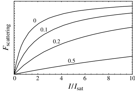
Figure 13.5 Scattering force for sodium atoms ( 1/\gamma = 16.1 ns, \lambda_0 = 590 nm) as a function of I/I_{\text{sat}} . The numbers on the curves indicate the frequency detuning in units of 10^7 (\omega - \omega_0)/\omega_0 .
