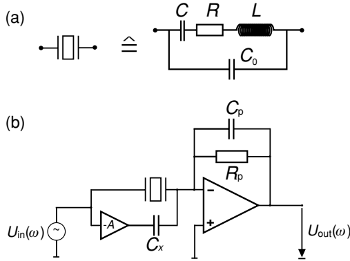
Figure 7.8 Equivalent electric circuit of a tuning fork and its measurement. (a) Symbol and Butterworth–Van-Dyke equivalent circuit. (b) Measurement of the tuning-fork admittance. The capacitor C_x and the gain of -A compensate for the tuning fork's stray capacitance C_0 .
