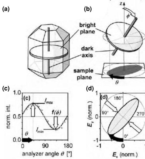
Figure 9.6 Degenerate emission dipole moment of a semiconductor nanocrystal. (a) Orientation of the bright plane and the dark axis within a CdSe nanocrystal. (b) If the crystal axis is tilted with respect to the normal of a supporting surface, the projection of the bright plane into this surface changes. (c) Light emitted by such a tilted nanocrystal is therefore only partially polarized. (d) From the absolute orientation and the ellipticity of the polarization ellipse, the 3D orientation of the dark axis can be determined. From [15].
