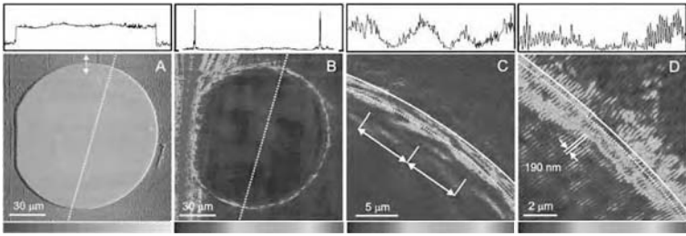
Figure 5.18 Field distribution near a micro-optical resonator imaged by photon tunneling microscopy. (A) topographic image of the disk-like resonator coupled to a waveguide (left). (B)–(D) STOM images of the field distribution for three different zoom levels showing mode beating in (C) and standing wave patterns with a periodicity of 190 nm in (D). Line cuts along the dotted lines for each image are shown in the top panels. The solid white line indicates the outline of the resonator rim. Adapted from [36].
