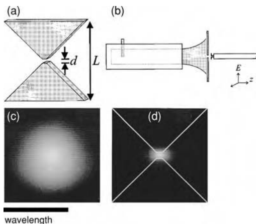
Figure 6.41 The bowtie antenna. (a) Geometrical outline of the antenna. (b) Experimental set-up used to demonstrate the performance at microwave frequencies. (c), (d) Measured intensity distribution without and with the antenna placed in front of the waveguide. Adapted from [78].
