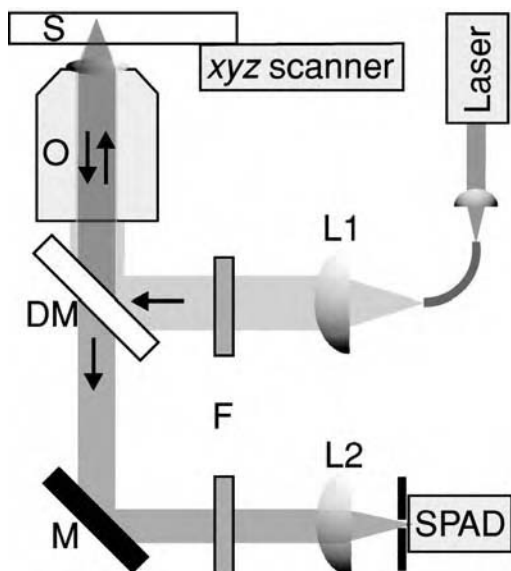
Figure 5.1 Set-up of a sample scanning epi-illumination confocal optical microscope. A laser light source is spatially filtered, e.g. by sending the light through a single-mode optical fiber or a pinhole. After exiting the fiber/pinhole the light is collimated by a lens. A (dichroic) beamsplitter reflects the light into a high-numerical-aperture microscope objective. The back-aperture of the objective should be overfilled to achieve the optimal spotsize (see Chapter 4). The optical signal (e.g. fluorescence) and scattered light created at the focus are collected by the same objective and converted into a collimated beam. The dichroic beamsplitter transmits light in a restricted spectral range, which is then filtered further and finally focused onto another pinhole in front of a detector. Images are obtained pixel by pixel by scanning the sample relative to the focus.
