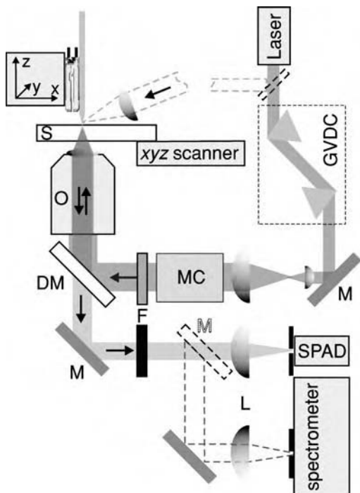
Figure 5.11 Nonlinear tip-enhanced near-field microscopy. GVDC: group velocity dispersion compensation M: minor, MC: mode converter, F: filter, DM: dichroic mirror, O: microscope objective, S: sample, L: lenses, SPAD: single-photon counting avalanche photodiode.
