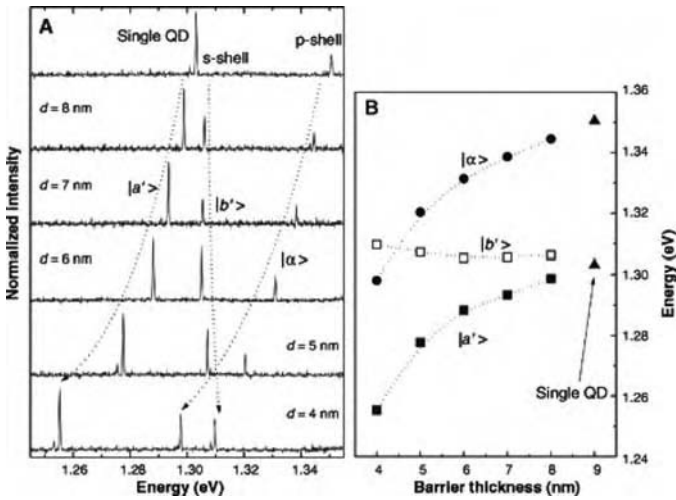
Figure 8.16 Level splitting of two InAs quantum dots separated by a GaAs barrier. (A) Emission spectra at T \approx 60 K for varying dot separation d . (B) Corresponding energy level diagram. From [35].
