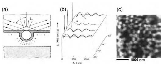
Figure 6.38 Particle plasmon probe. (a) A polystyrene bead on a flat glass substrate is covered with a 20 nm gold layer and illuminated in the Kretschmann configuration. The scattering of the protrusion is recorded as a sample is approached from the other side. (b) Recorded scattering intensity versus particle-surface distance for both p- and s-polarization. (c) Image recorded in constant height mode using electron tunneling feedback. Adapted from [72].
