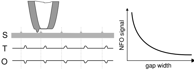
Figure 7.13 Near-field optical imaging on a sample with small topographic variations. Left panel: S, sample profile; T, apparent topography as measured by the probe; O, detected optical signal resulting from the particular probe-sample distance dependence (right panel).
