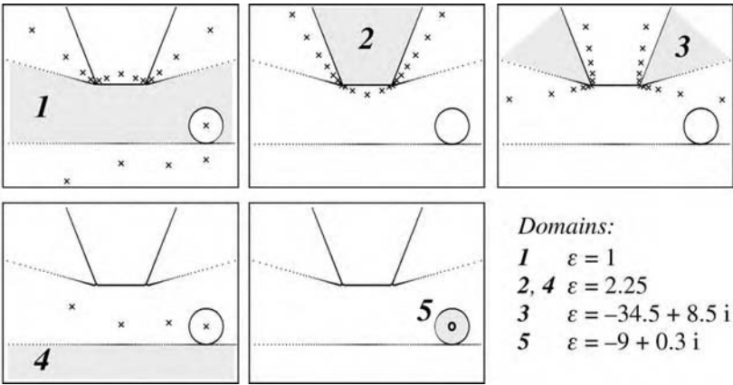
Figure 15.3 MMP model of a two-dimensional aperture-type near-field optical microscope. The locations of the multipole origins for the respective shaded domains are indicated by small crosses. Domain 5 is expanded by a normal expansion. The structure consists of a vacuum gap (1), a truncated glass wedge (2) embedded in an aluminum screen (3), a planar transparent glass substrate (4) carrying a cylindrical silver particle (5).
