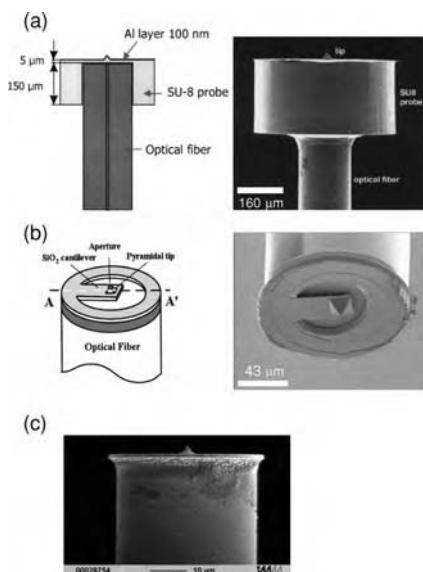
Figure 6.27 Microfabricated probes based on optical fibers. (a) Microfabricated photoplastic probe attached to the end of a single mode fiber. From [48]. (b) Hybrid optical fiber probe. From [49]. (c) Another example adapted from [50].
