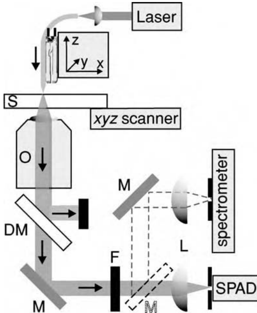
Figure 5.10 Typical set-up for a fluorescence aperture scanning near-field optical microscope. Note the similarity to the confocal set-up in Fig. 5.1. Laser light is injected into an optical fiber that holds an optical probe at its far end. The probe is held within near-field distance of the sample using e.g. a tuning-fork shear-force feedback (see Chapter 7). The light interacts with the sample and is collected by a microscope objective that is aligned with respect to the fiber axis. In the case of fluorescence imaging, a dichroic mirror reflects most of the excitation light. Residual excitation light is removed by additional filters and the redshifted fluorescence is focused onto a detector or spectrometer. M: mirrors, L: lenses, DM: dichroic mirror. The dashed mirror can be flipped in and out of the beam path.
