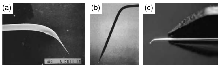
Figure 7.11 Cantilevered fiber probes. (a) Bent fiber probe with a mirror facet for beam deflection. The resonant frequency of the cantilevered probe is \sim 14 kHz and the Q -factor is \sim 30 in water, sufficient to perform near-field imaging on soft samples in liquid cells. From [21]. (b) Different type of bent fiber probe. The resonances are typically in the range of 30 to 60 kHz, the Q -factors are larger than 100, and the measured spring constants are 300 to 400 N/m. From [22]. (c) Commercially available cantilevered fiber probe from Nanonics.
