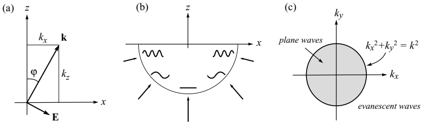
Figure 2.10 (a) Representation of a plane wave propagating at an angle \varphi to the z axis. (b) Illustration of the transverse spatial frequencies of plane waves incident from different angles. The transverse wavenumber (k_x^2 + k_y^2)^{1/2} depends on the angle of incidence and is limited to the interval [0 \dots k] . (c) The transverse wavenumbers k_x, k_y of plane waves are restricted to a circular area with radius k . Evanescent waves fill the space outside the circle.
