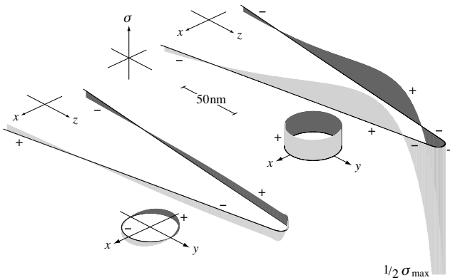
Figure 6.33 Induced surface charge density corresponding to Fig. 6.32(a) (left) and Fig. 6.32(b) (right). The surface charges form a standing wave in each case. In (a) the surface charge wave has a node at the end of the tip, whereas in (b) there is a large surface charge accumulation at the foremost part, responsible for the field enhancement.
