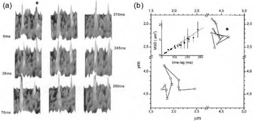
Figure 4.15 Tracing fast diffusion with subwavelength accuracy. (a) Series of 5 ms exposures recorded at 35 ms intervals of two fluorescence peaks of individual labelled lipids in a lipid bilayer. Image size: 5.4 \times 5.4 \mu\text{m}^2 . (b) Trajectories of both molecules as obtained by fitting the peaks in (a). Inset: Mean-square displacement of individual molecules averaged over many trajectories. Adapted from Ref. [18].
