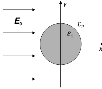
Figure 12.16 Cut through a thin wire that is illuminated by an x -polarized plane wave.
