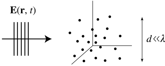
Figure 14.1 Interaction of an optical field with a system of particles initially at thermal equilibrium. The state of the system is defined by the phase-space coordinate s = [q_1 \dots q_N; p_1 \dots p_N] , with q_j and p_j being the coordinates and conjugate momenta, respectively. If the characteristic length scale d of the system is small compared with the wavelength \lambda , the interaction energy between the optical field and the system is given by the electric dipole approximation \delta H = -\boldsymbol{\mu}(s, t) \cdot \mathbf{E}(t) , where \boldsymbol{\mu} is the electric dipole moment.
