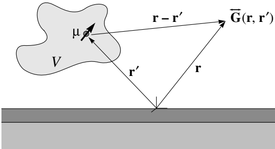
Figure 15.5 Illustration of the dyadic Green's function \vec{\mathbf{G}}(\mathbf{r}, \mathbf{r}') . \mathbf{r}' and \mathbf{r} represent the dipolar source and the point of observation, respectively. The field at \mathbf{r} depends on the orientation of the dipole at \mathbf{r}' . The three columns of \vec{\mathbf{G}} denote the electric fields for the three major orientations of the dipole.
