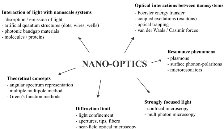
Figure 1.2 Constituents of the field of nano-optics.
