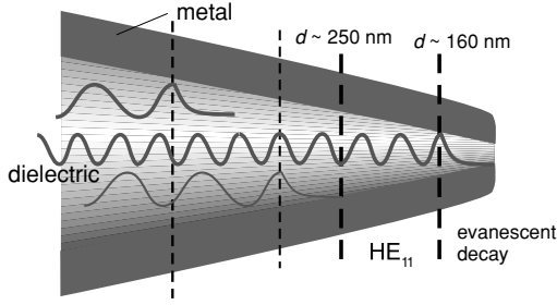
Figure 6.9 Cartoon of the successive cut-off of guided modes and exponential decay of the fields towards the aperture in a tapered, metal-coated waveguide. Adapted from [17].
