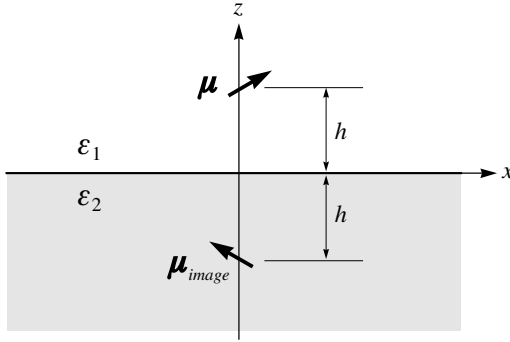
Figure 10.11 Principle of the image dipole approximation. \mu and \mu_{\text{image}} denote the primary dipole and the image dipole, respectively. Static image theory is applied to determine the magnitude of \mu_{\text{image}} .
