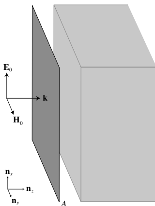
Figure 13.2 Configuration used to derive the radiation pressure.
