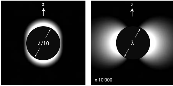
Figure 8.4 Electric energy density outside a fictitious sphere enclosing a dipole \mu = \mu_z . (Left) Close to the dipole's origin the field distribution is elongated along the dipole axis (near-field). (Right) At larger distances the field spreads transverse to the dipole axis (far-field).
