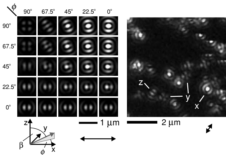
Figure 9.16 Left panel: Calculated fluorescence rate patterns for a focused annular beam probed by molecules with varying orientations of the dipole moment. Right panel: Experimental patterns. Each of these patterns can be assigned to a specific orientation of the molecular absorption dipole. The arrow indicates the polarization direction. Adapted from [24].
