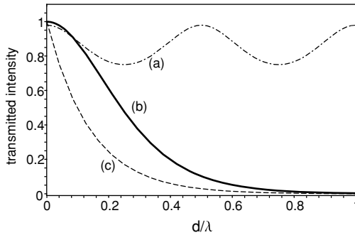
Figure 2.8 Transmission of a system of three media with parallel interfaces as a function of the gap d between the two interfaces. A p-polarized plane wave excites the system. The material constants are n_1 = 2 , n_2 = 1 , n_3 = 1.51 . This leads to critical angles \theta_c of 30^\circ and 49.25^\circ . For angles of incidence \theta_i between (a) 0^\circ and 30^\circ the gap dependence shows interference-like behavior (here \theta_i = 0^\circ , dash-dotted line), for angles between (b) 30^\circ and 49.25^\circ the transmission (monotonically) decreases with increasing gap width (here \theta_i = 35^\circ , full line). (c) Intensity of the evanescent wave in the absence of the third medium.
