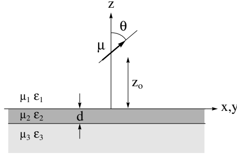
Figure C.1 An electric dipole with moment \mu is located at \mathbf{r}_0 = (0, 0, z_0) near a layered substrate. The fields in each medium are expressed in cylindrical coordinates \mathbf{r} = (\rho, \varphi, z) .
