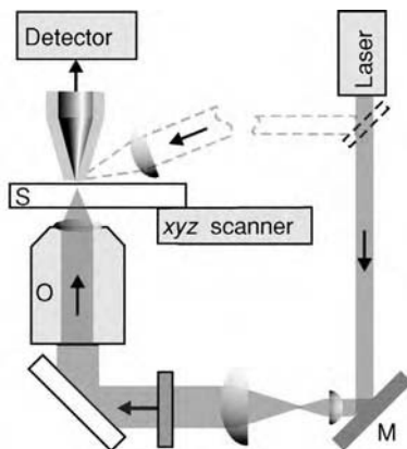
Figure 5.23 Collection mode SNOM: The sample is illuminated with a focused laser beam in reflection or transmission geometry. An aperture probe is used to locally pick up a light signal out of the sample's near-field. The signal is recorded by a detector at the far end of the fiber.
