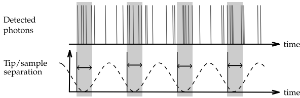
Figure 5.16 Correlation of photon arrival times with the vertical oscillation of the near-field probe. In time-stamping only photons that fall into periodic time-windows (shaded areas) with preset widths (arrows) are counted.
