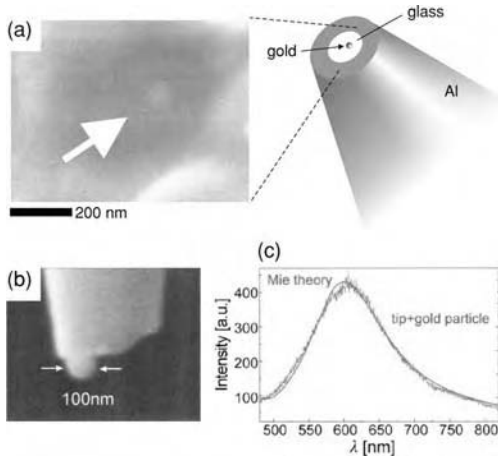
Figure 6.40 Particle plasmon tips: (a) Chemically grafted gold particle (diameter \sim 60 nm) in the aperture (diameter \sim 200 nm) of an aluminum-coated silica tip. Adapted from [76]. (b) Chemically grafted 100 nm gold particle at the apex of a dielectric fiber probe. (c) Spectrum of the light scattered off the particle tip in (b). (b) and (c) adapted from [77].
